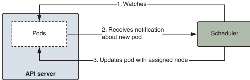
Figure 9.12 The scheduler watches the API server for newly created pods and determines which node they should run on.
