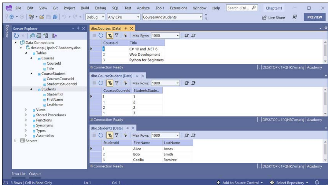
Figure 10.6: Viewing the Academy database in SQL Server using Visual Studio 2022 Server Explorer
