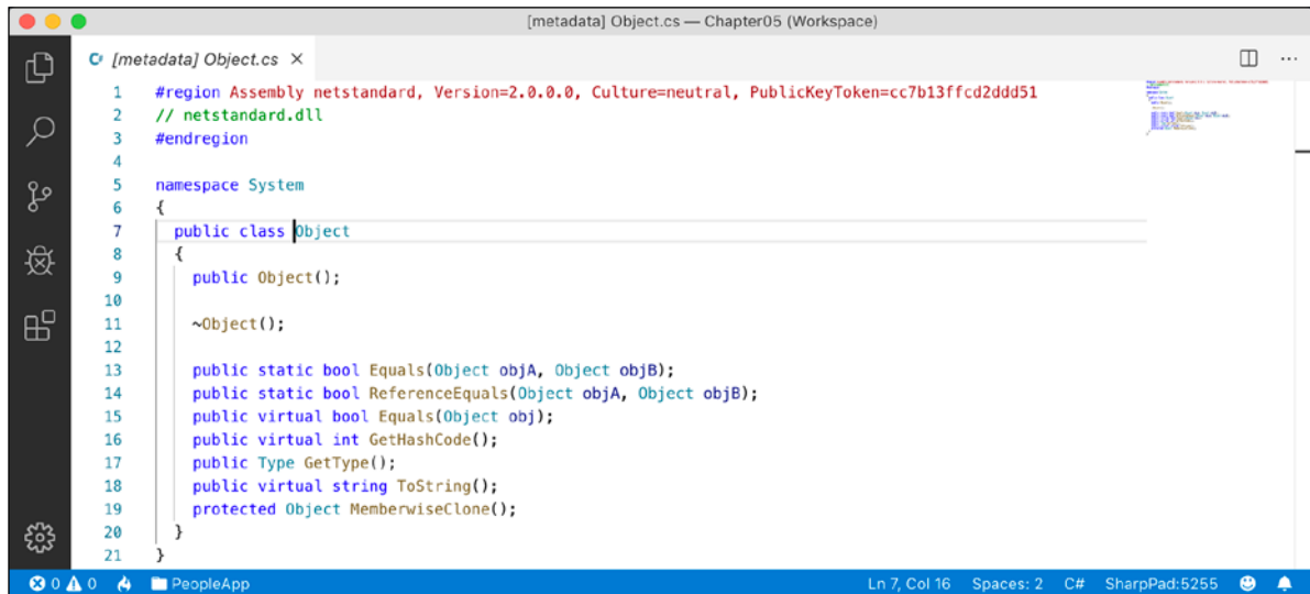
Figure 5.1: System.Object class definition
