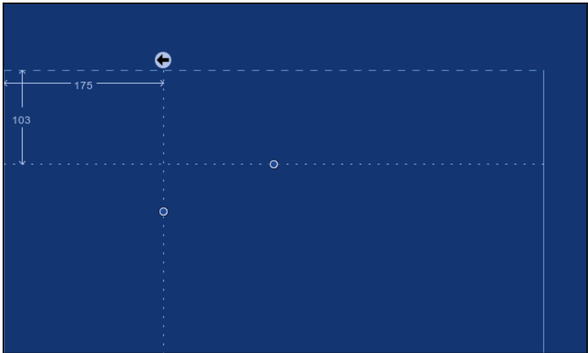
Constraint guidelines
