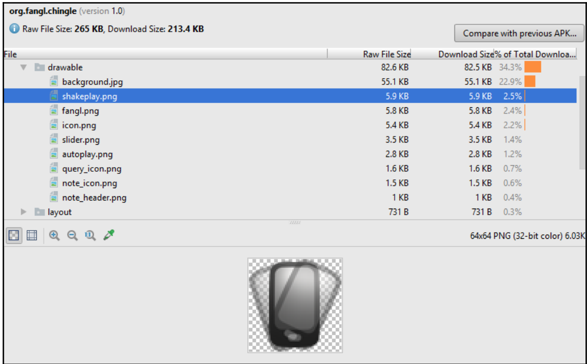
APK analysis
