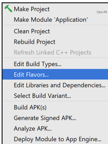
Build options
