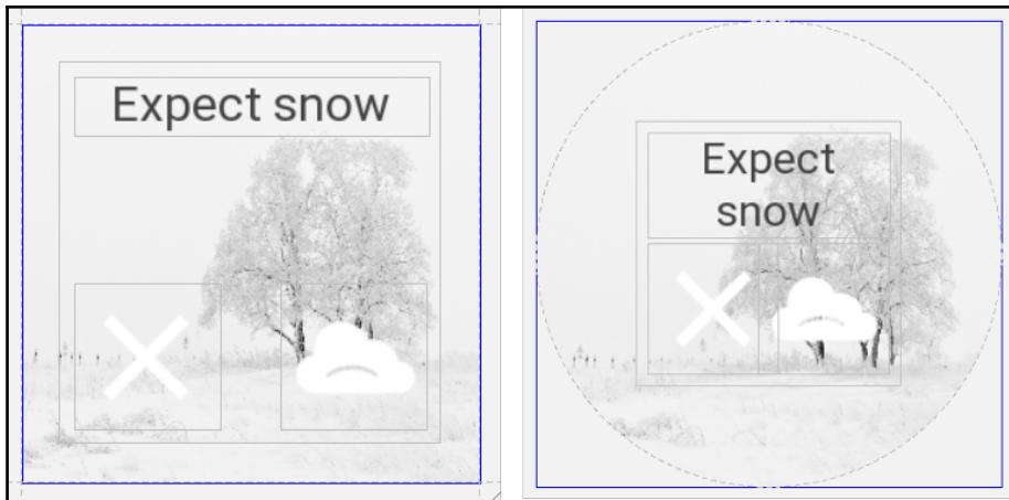
The BoxInsetLayout
