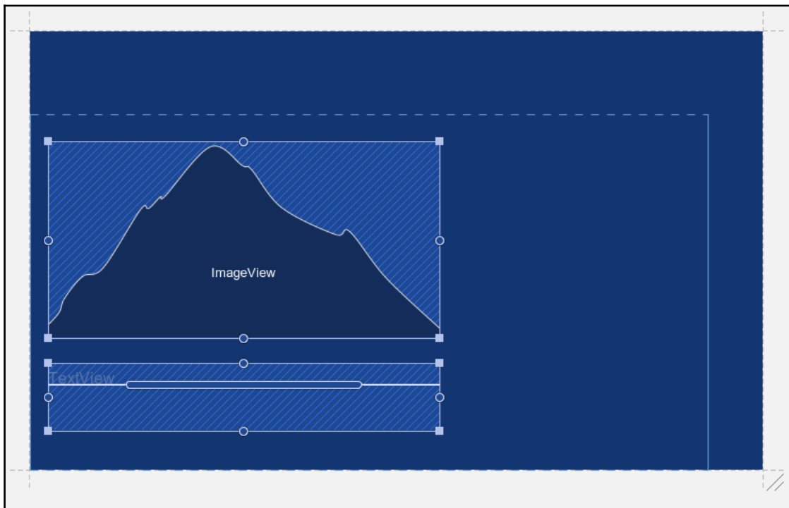
Constraint handles
