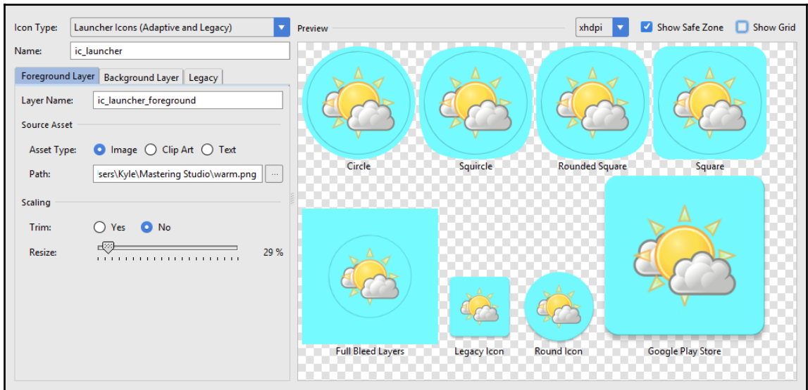
Asset Studio
