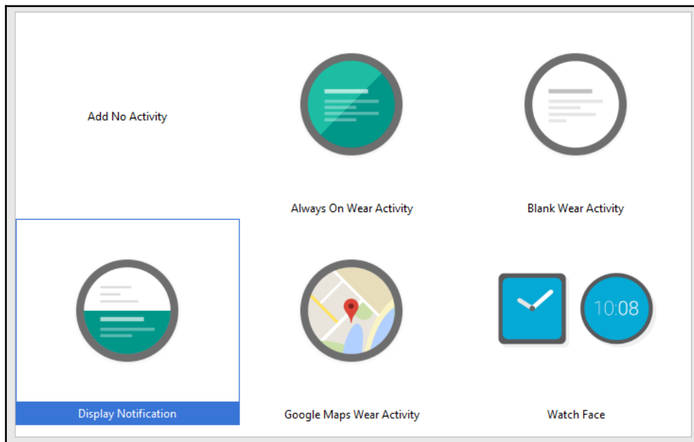
Wear templates
