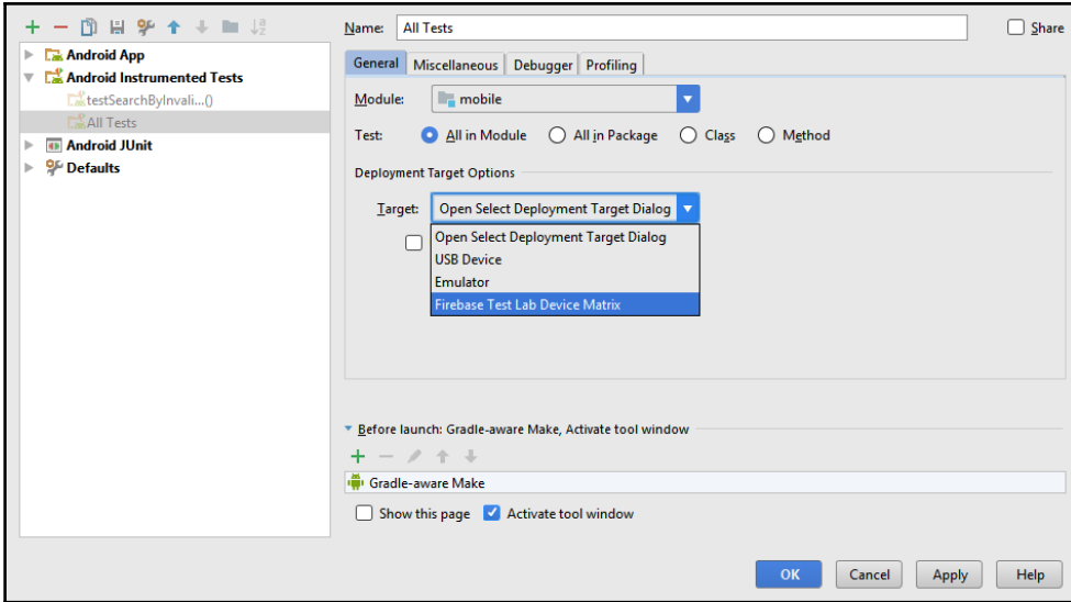
Test configuration
