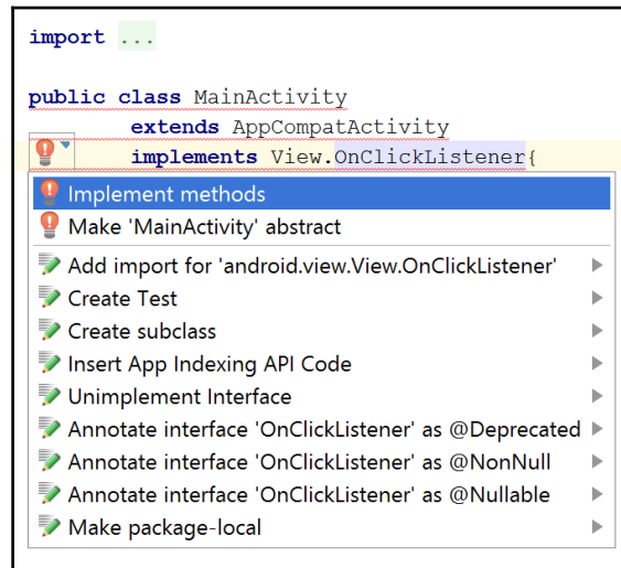
Quick fix
