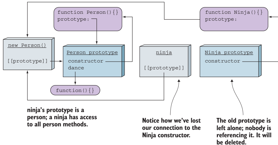
Figure 7.14 We've achieved inheritance by setting the prototype of the Ninja constructor to a new instance of a Person object.
