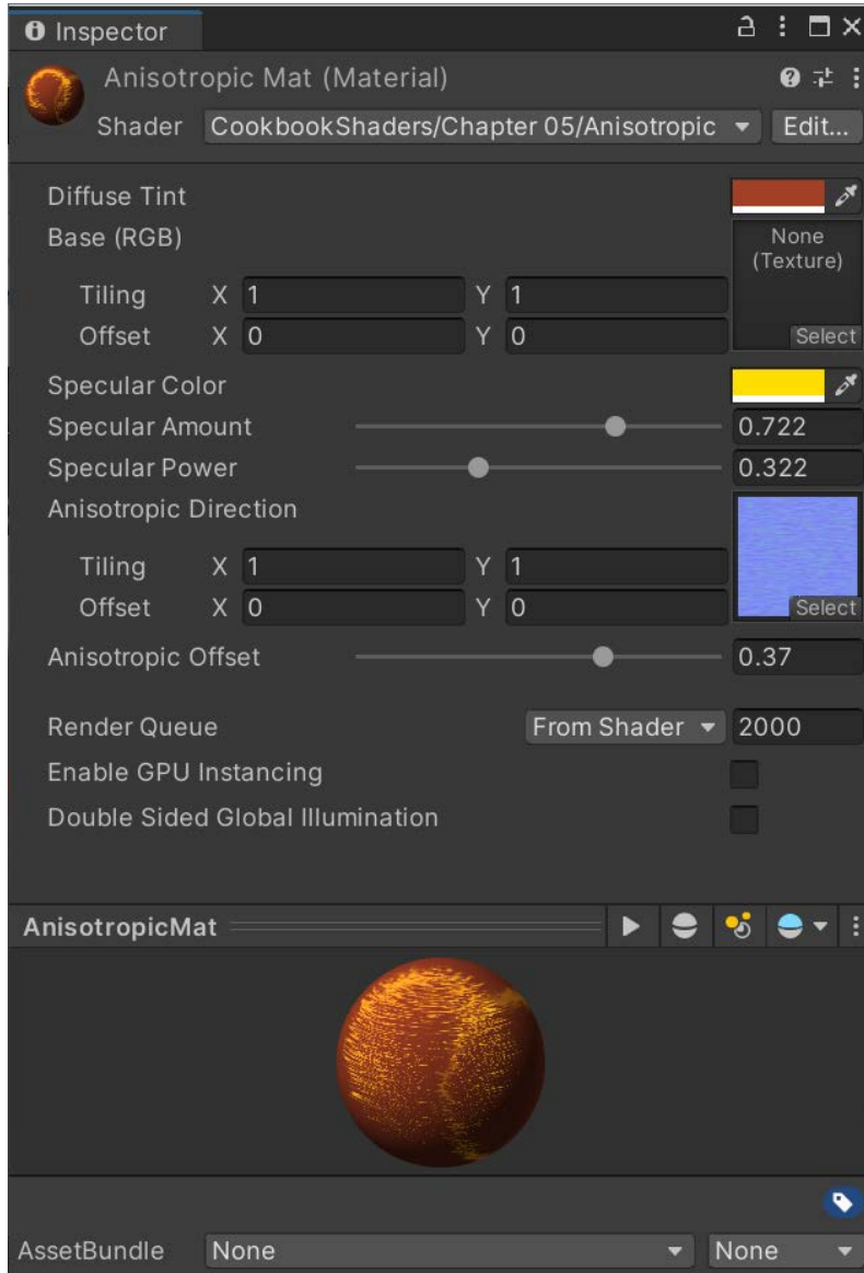
Figure 5.28 – Tweaked parameters within the Anisotropic Material
