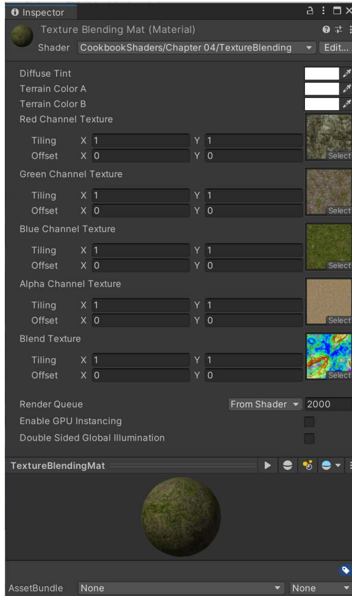
Figure 4.18 – Assigning the textures to be blended
