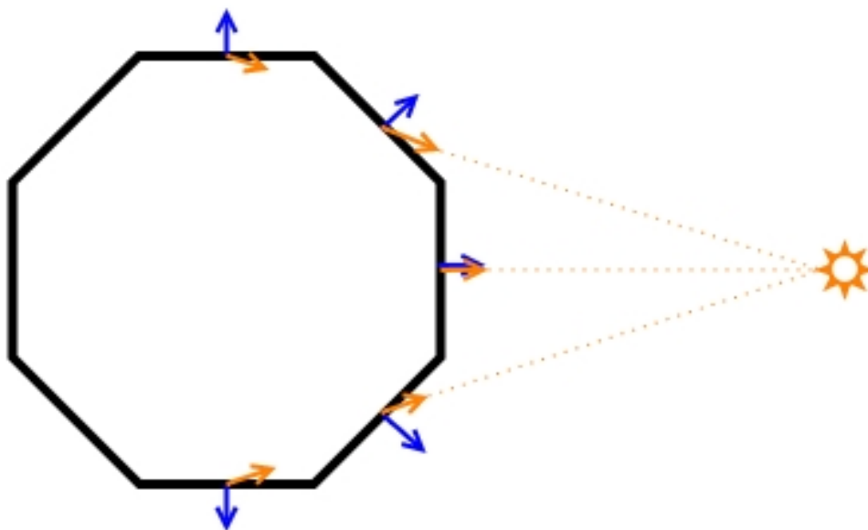
Figure 5.6 – A demonstration of the Lambertian model
