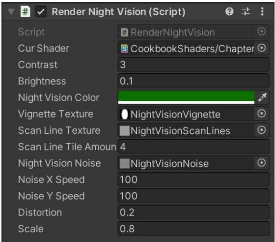
Figure 11.14 – The settings for the night-vision script
