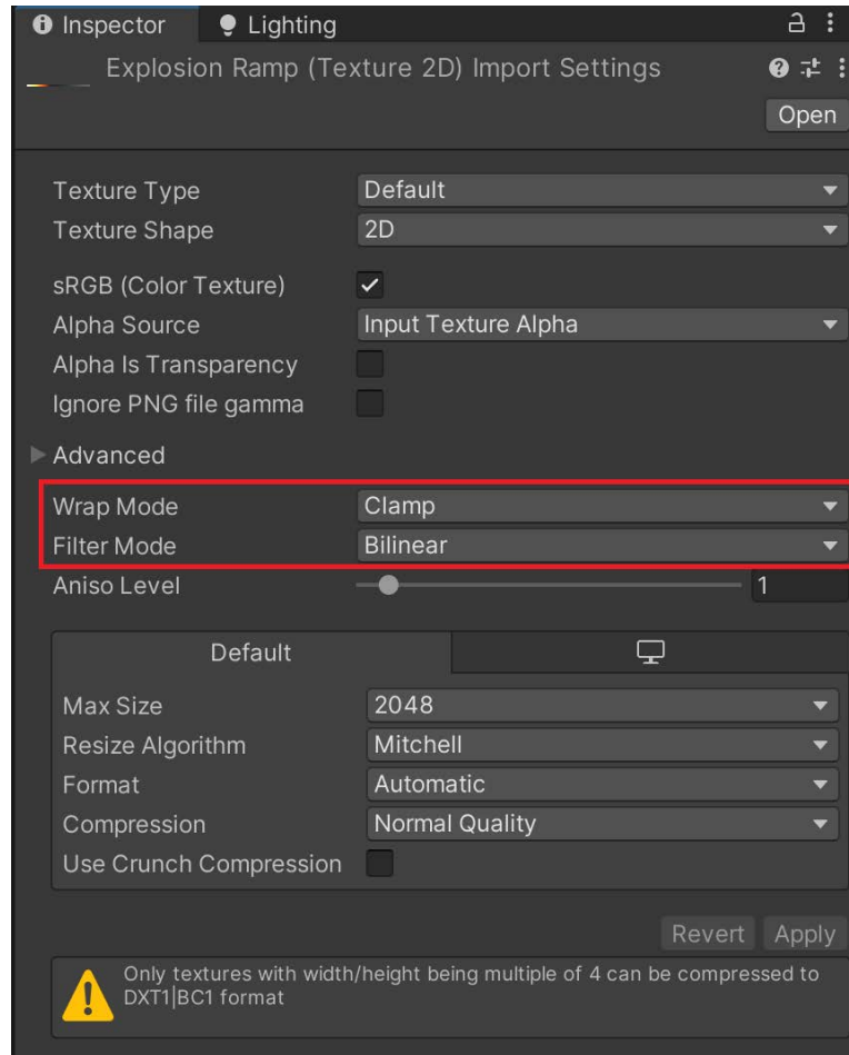
Figure 7.15 – Setting the Wrap Mode and Filter Mode properties
