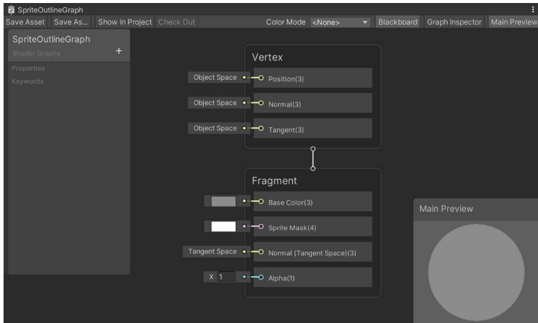
Figure 13.27 – The sprite graph open
