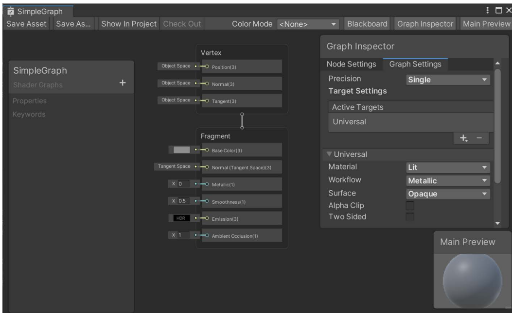
Figure 13.9 – The Shader Graph editor
