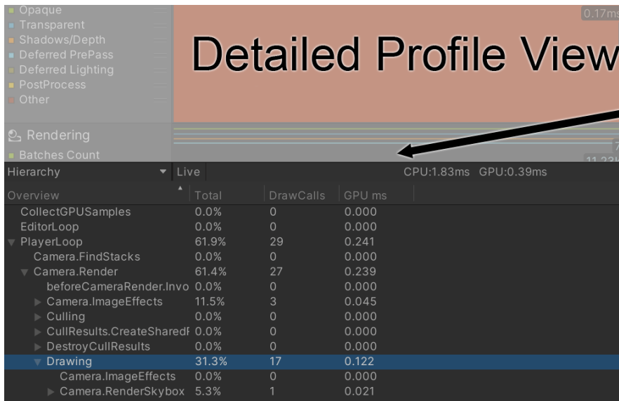
Figure 9.11 – Detailed Profile View
