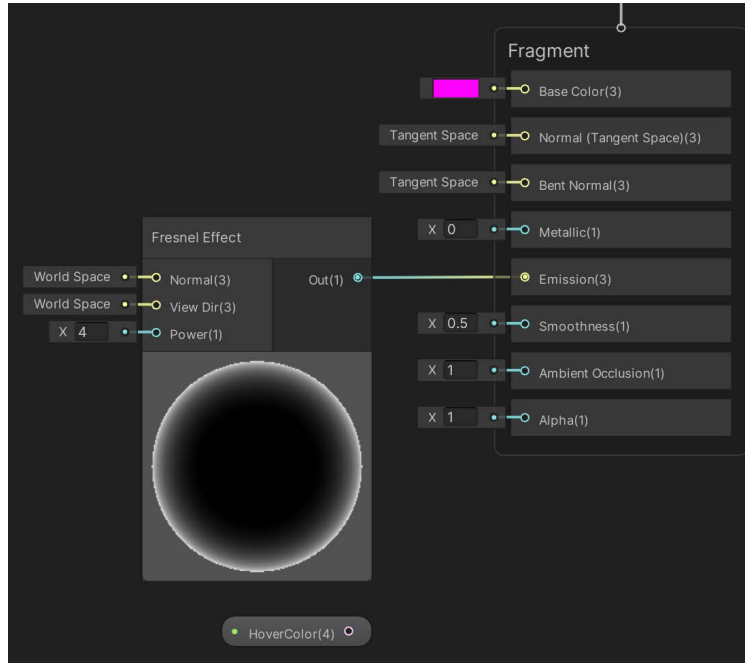
Figure 14.5 – Fresnel Effect node
