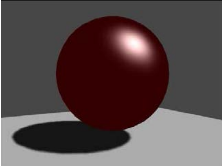
Figure 5.21 – The final result of our Phong Specular calculation
