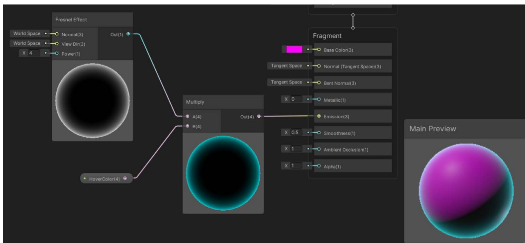
Figure 14.6 – Multiplying the Fresnel Effect with a color
