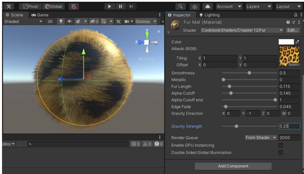
Figure 12.14 – Adjusting the properties on the fur shader
