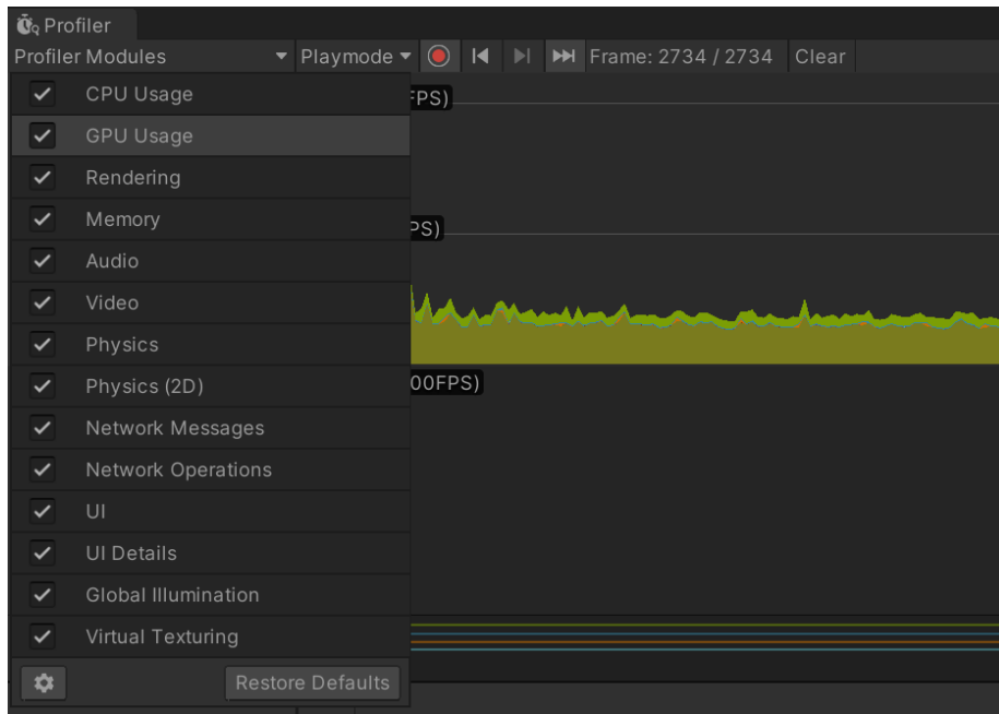
Figure 9.8 – Enabling the GPU Usage panel
