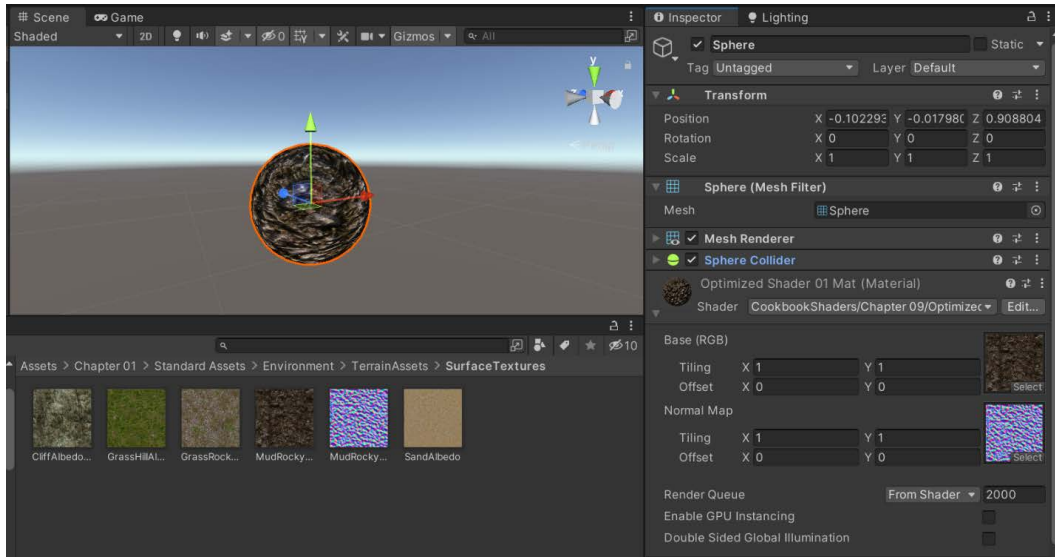
Figure 9.2 – Assigning a texture and normal map to the material
