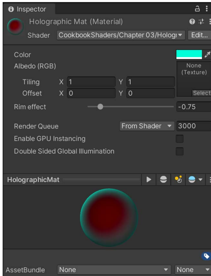
Figure 3.15 – Adjusting the Color and Rim effect properties
