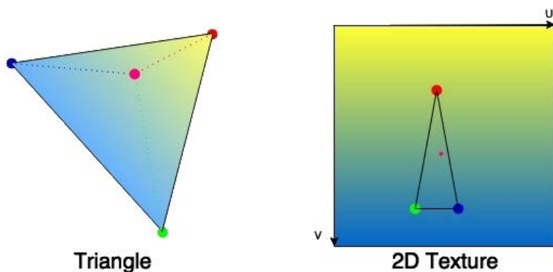
Figure 4.1 – How UVs are projected to a polygon
