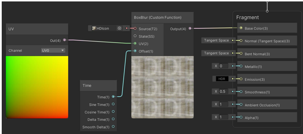
Figure 14.21 – Connecting the BoxBlur Custom Function node to Fragment
