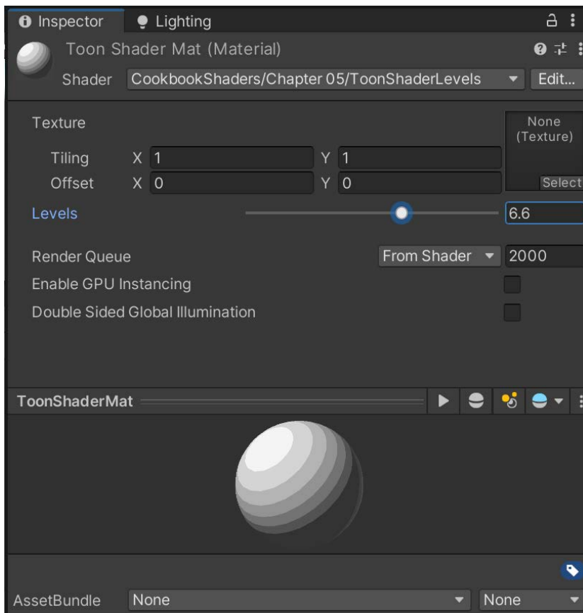
Figure 5.15 – Adjusting the Levels property
