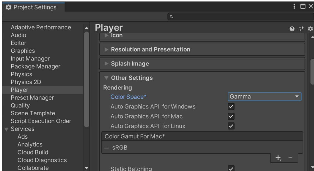
Figure 12.5 – Location of the Color Space property
