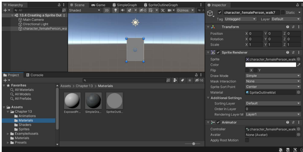
Figure 13.26 – The gray sprite
