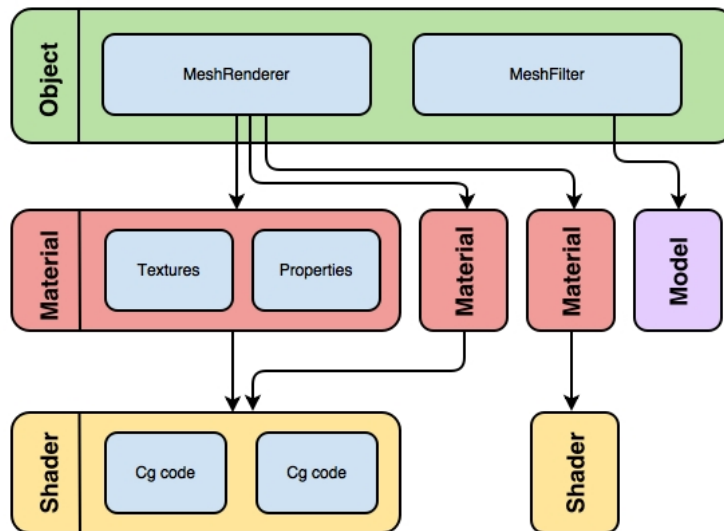
Figure 2.1 – Relationship between shaders, models, materials, and objects
