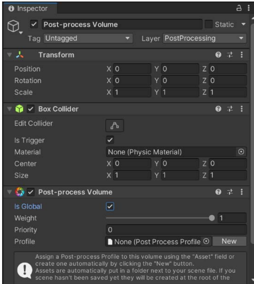
Figure 1.13 – Assigning the Is Global property
