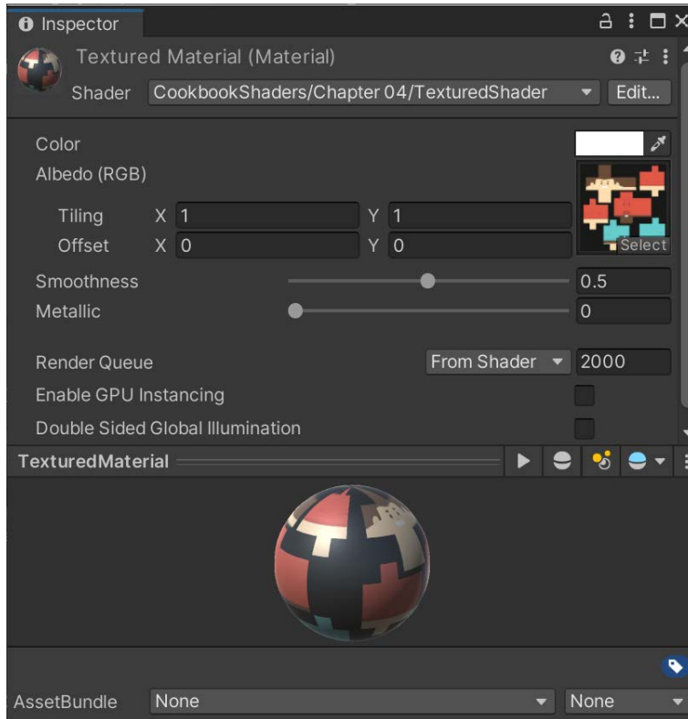
Figure 4.3 – The finished Textured Shader
