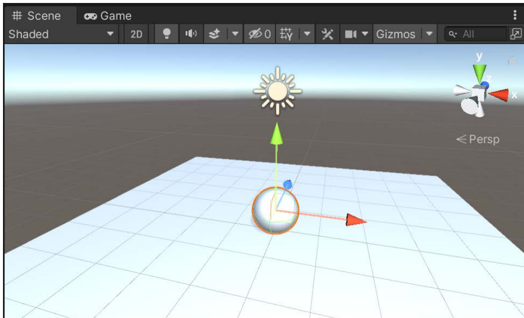
Figure 5.23 – The results of the Blinn-Phong lighting model
