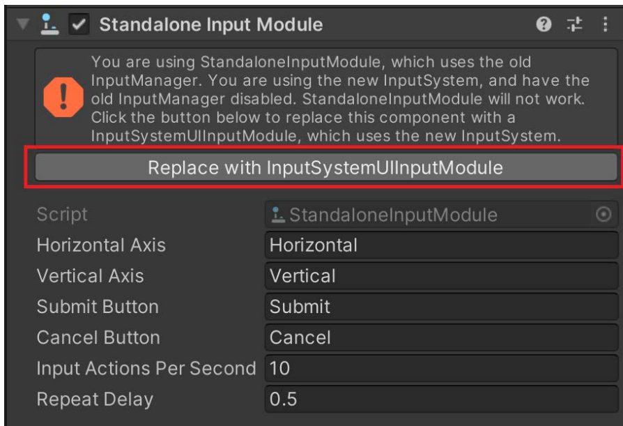
Figure 14.10 – The original Event System has this component of the old Input System
