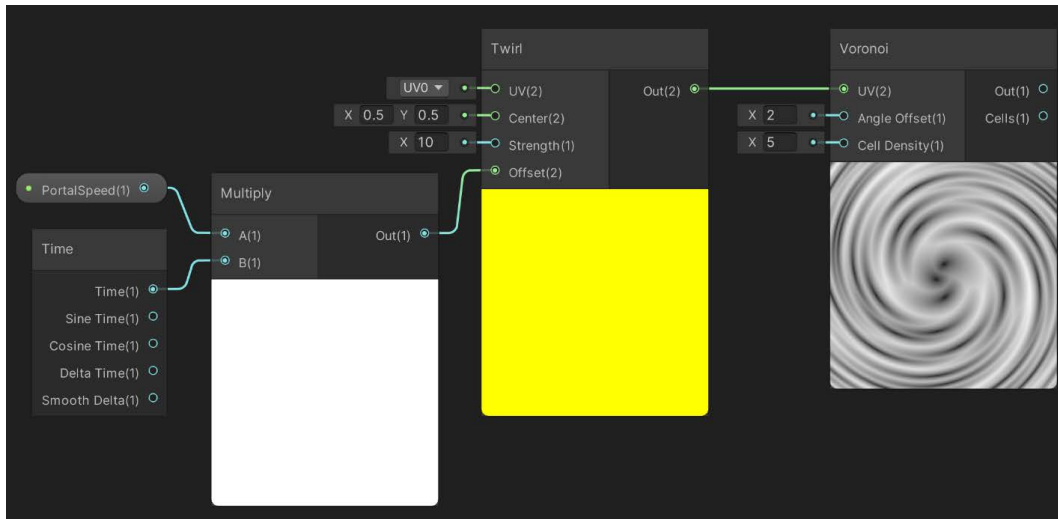
Figure 14.15 – Moving portal texture
