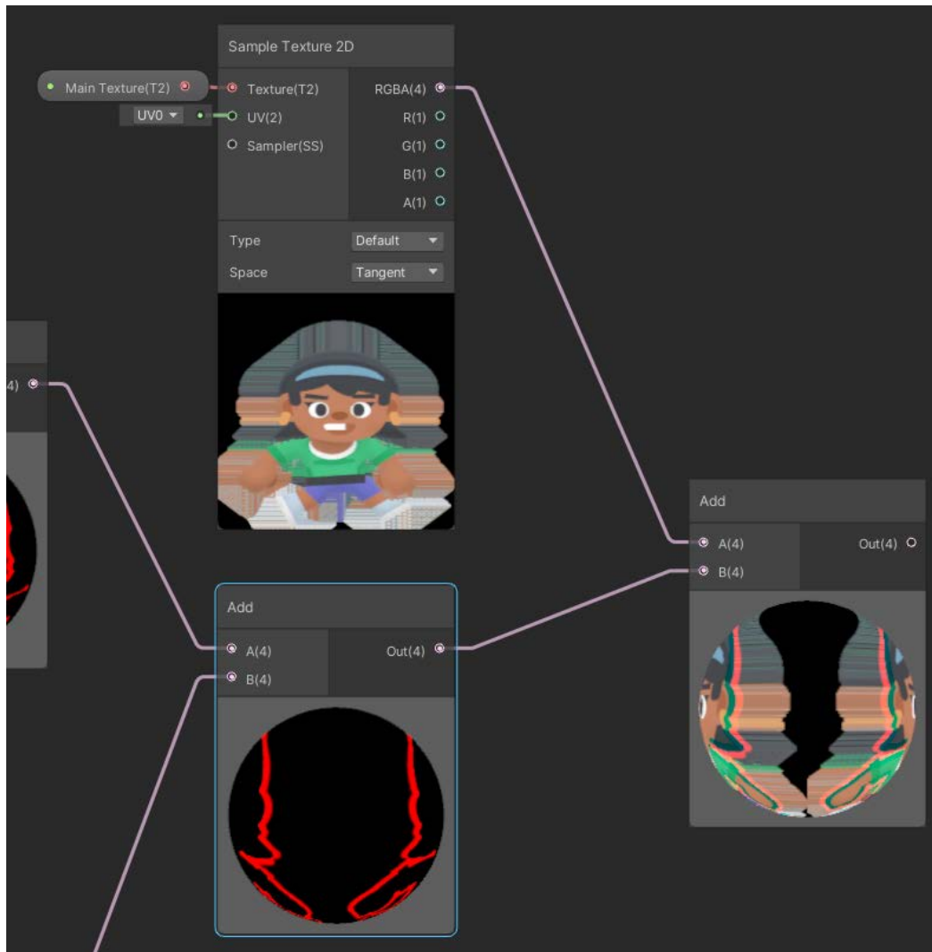
Figure 13.46 – Adding the edge and the original texture
