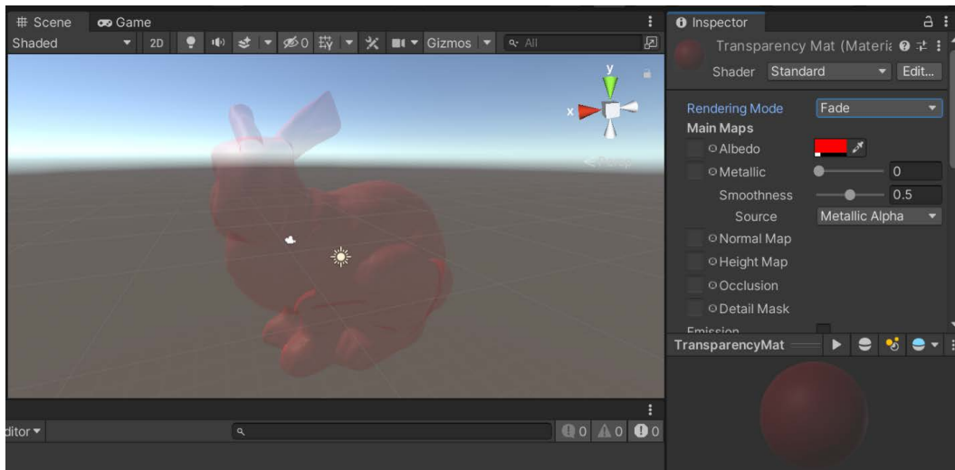
Figure 6.9 – Changing Rendering Mode to Fade
