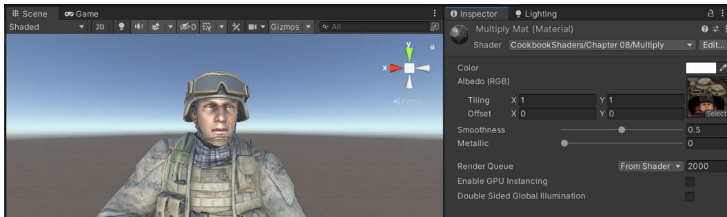
Figure 8.3 – Adding the texture to the Albedo (RGB) property
