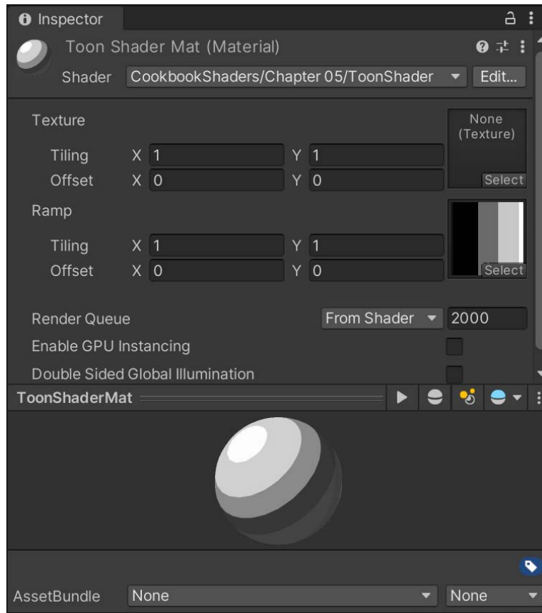
Figure 5.11 – The Toon Shader material with the Ramp texture applied
