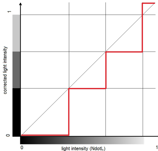
Figure 5.14 – How a ramp map is used to correct the light intensity
