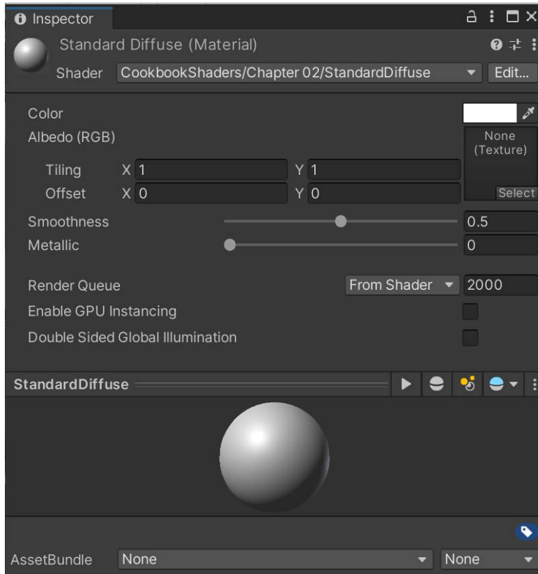
Figure 2.7 – The StandardDiffuse shader has been set as the shader to use on this material
