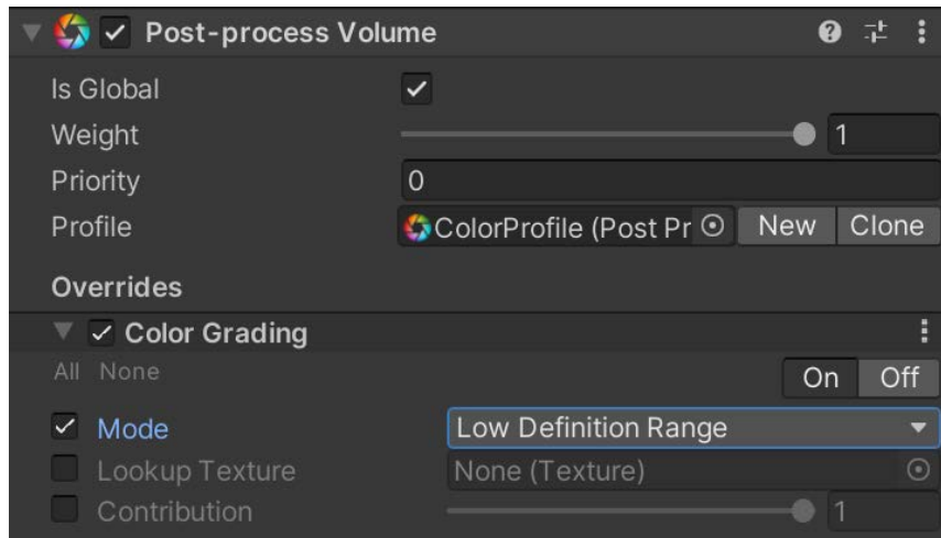
Figure 1.32 – Assigning Low Definition Range for Mode
