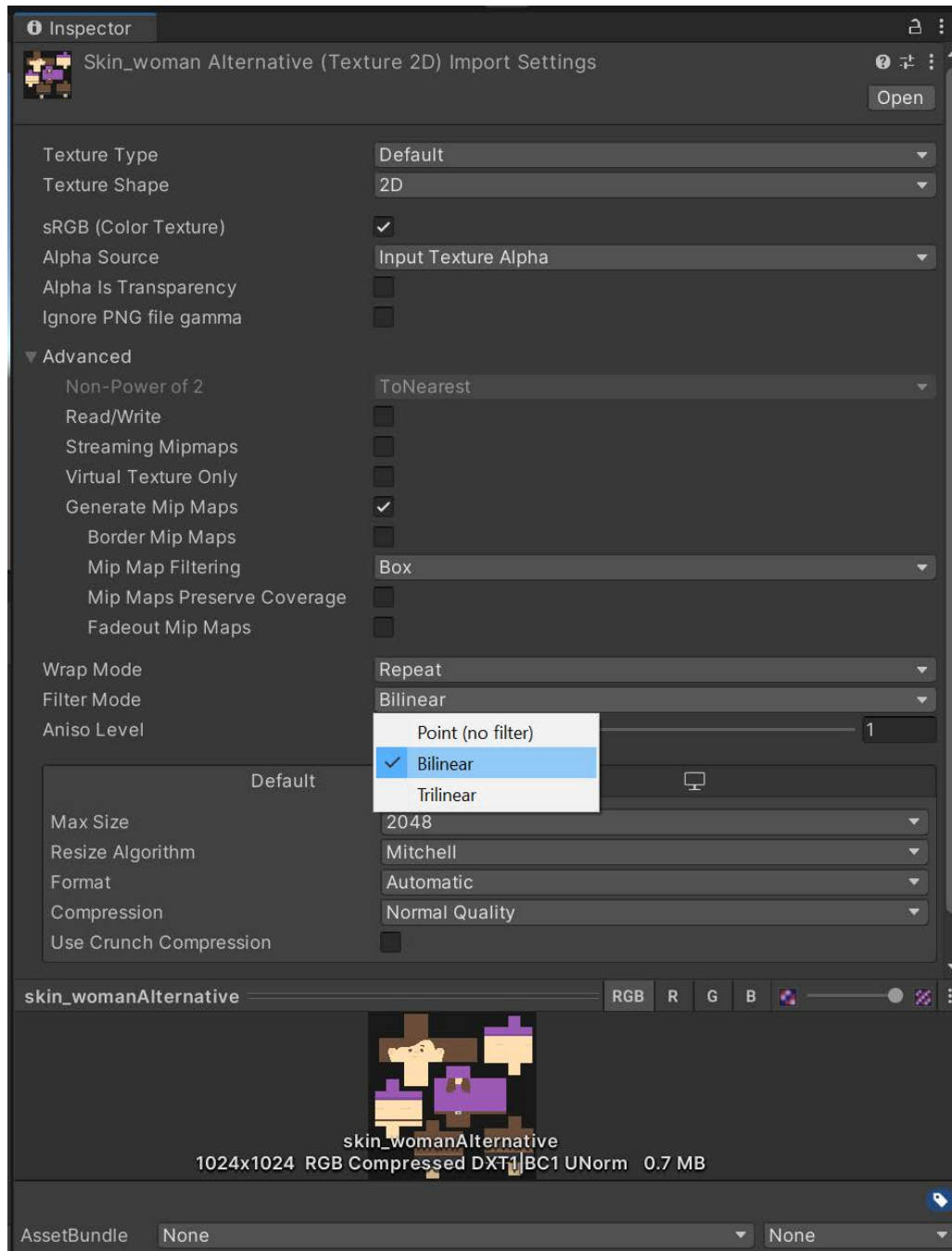
Figure 4.7 – The location of Filter Mode, set to Bilinear
