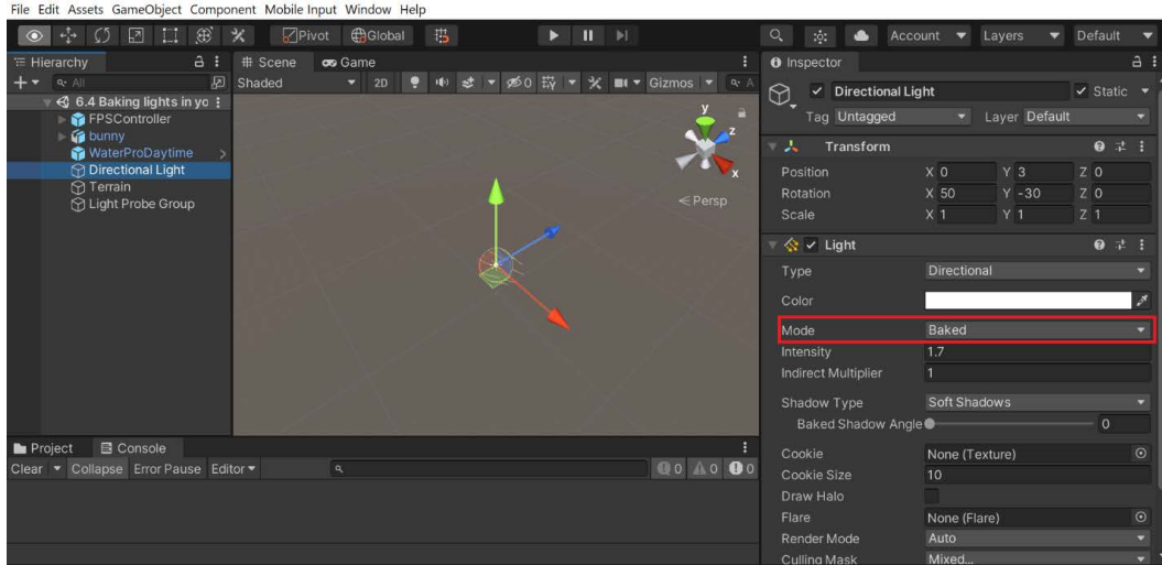
Figure 6.22 – Setting the light's Mode to Baked
