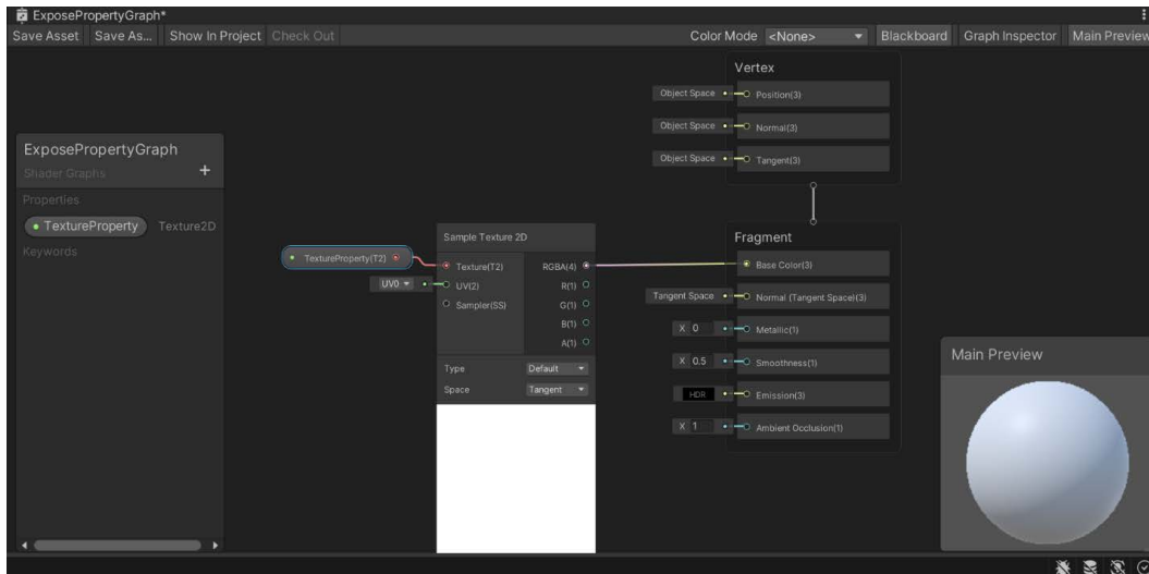
Figure 13.19 – Adding the texture property to the node
