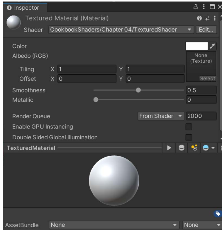
Figure 4.2 – The Shader assigned
