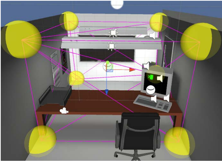
Figure 6.19 – How light probes can be used to enclose the volume of a static office space For our example, it would just be the center area that the player can enter:
