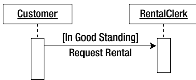
Figure 3-7. Identifying conditional constraints
