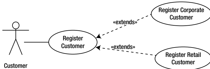
Figure 2-4. Extending use cases
