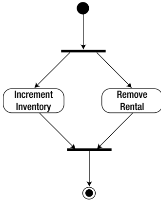
Figure 3-18. Parallel processing depicted in an activity diagram
