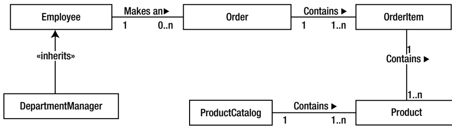
Figure 4-9. The Purchase Request component class diagram with associations added
