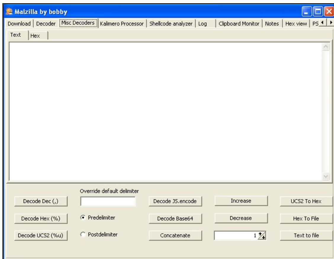
Figure 16: Malzilla decoders
