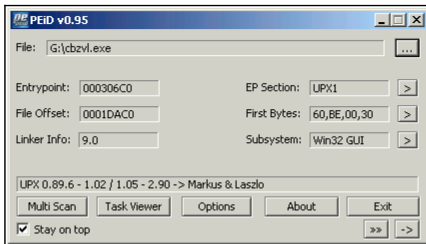
Figure 5: PEID UI
