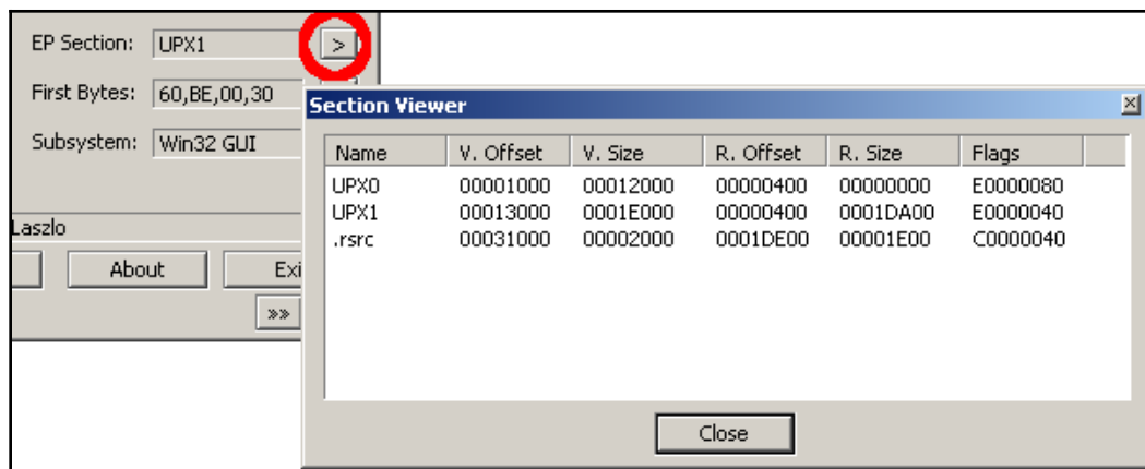
Figure 3: PEiD tool's section viewer
