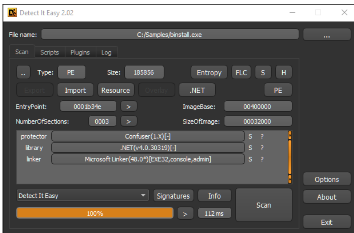
Figure 12: Detect it Easy for detecting the obfuscator (ConfuserEx)
