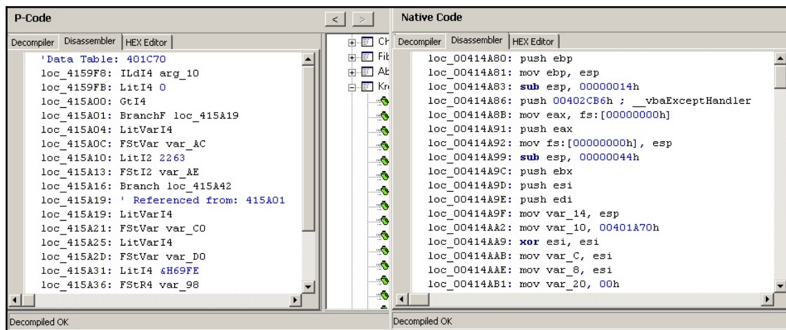
Figure 17. P-code versus native code samples in VB Decompiler Lite
