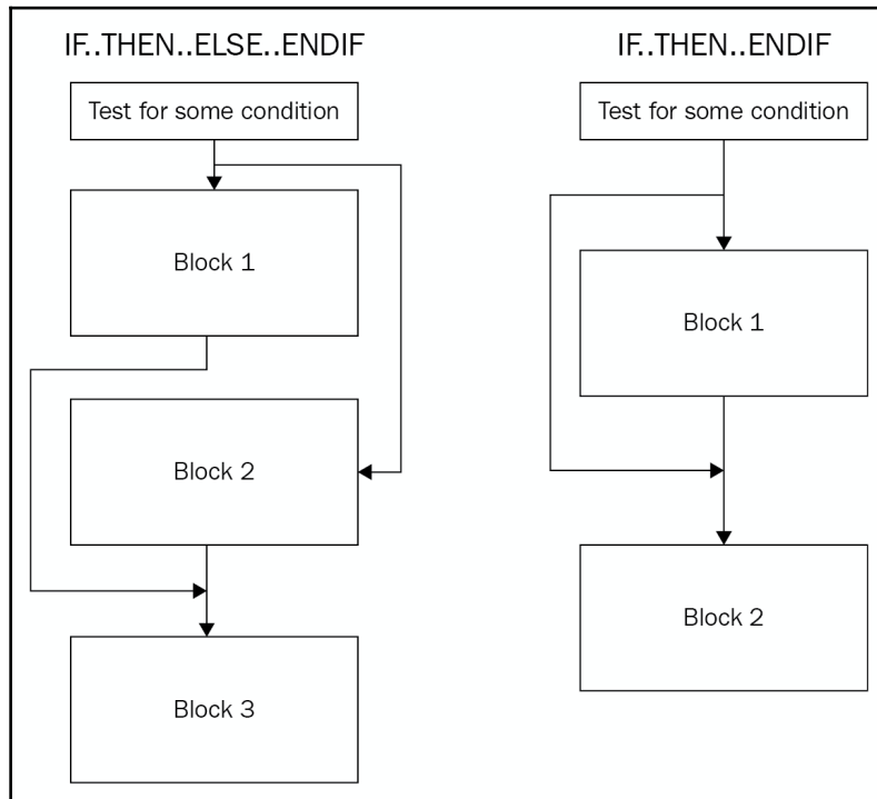
Figure 7: Conditional flow redirection
