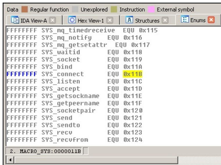
Figure 3: ARM syscall mappings in IDA
