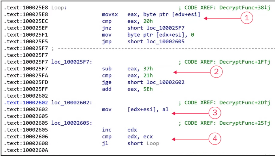
Figure 24: Things to pay attention to when identifying the encryption algorithm
