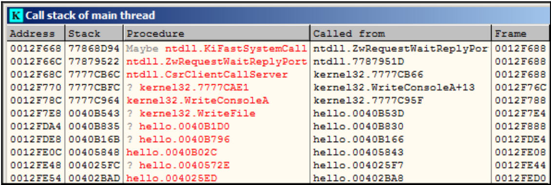
Figure 11: Call stack window in OllyDbg
