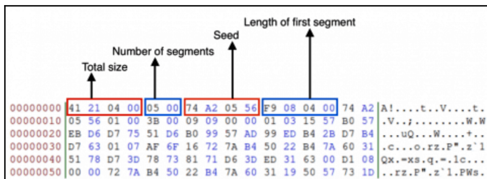
Figure 35: The structure used for decryption in the Vawtrak malware
