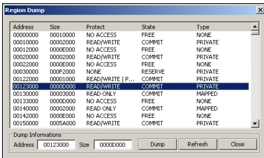
Figure 17: Region Dump window of PETools
