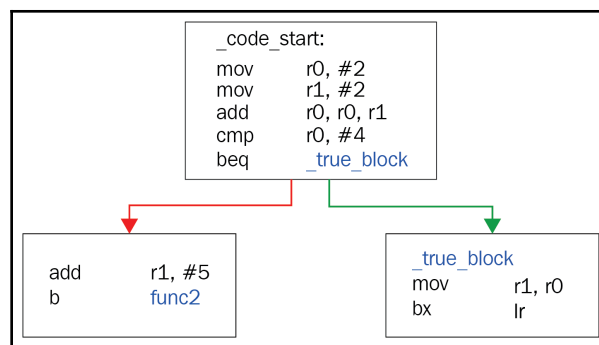
Figure 2: An example of a conditional jump
