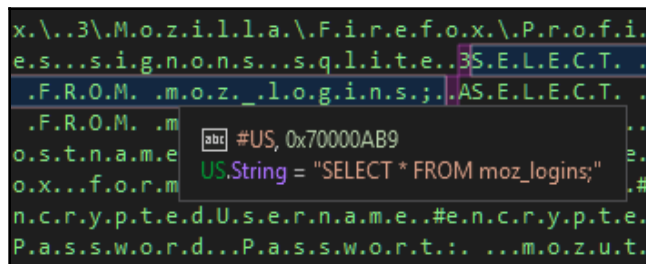
Figure 4: #US unicode string started with the length and followed by the actual string
