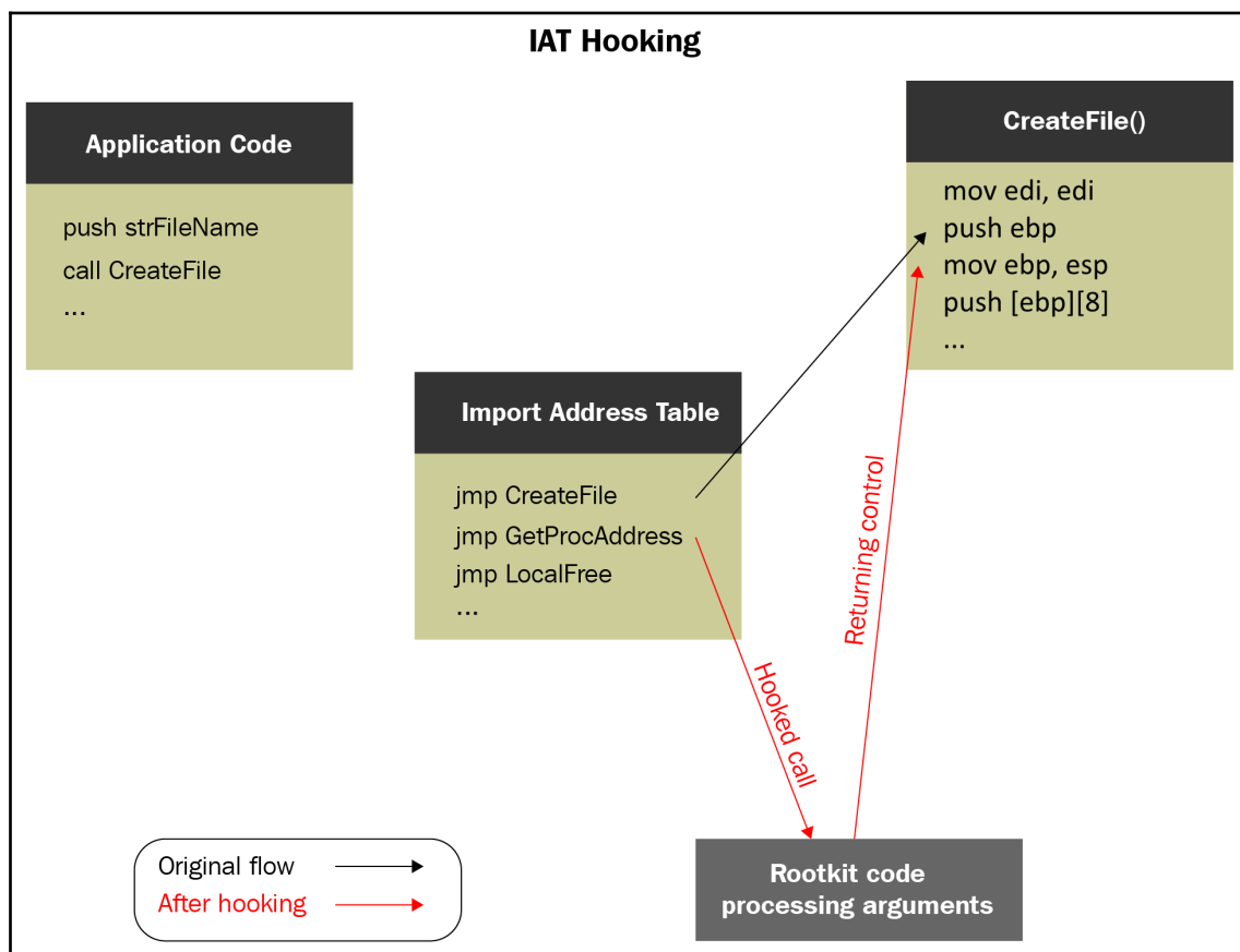
Figure 20. IAT hooking mechanism
