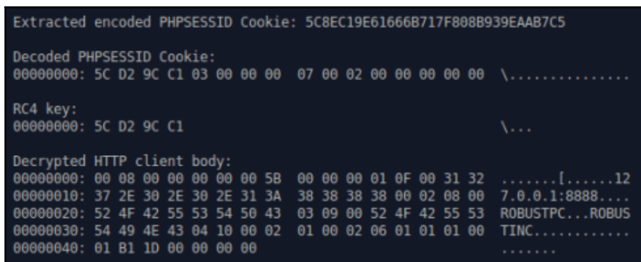
Figure 34: Extracted information from the network traffic of the Vawtrak malware
