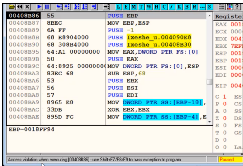
Figure 9: Staying at the OEP of the sample in OllyDbg
