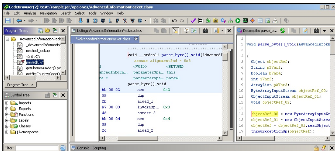
Figure 22: Disassembled and decompiled Java bytecode in Ghidra
