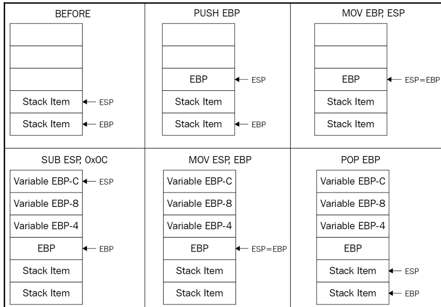
Figure 4: An example of a stack change at the beginning and at the end of the function
