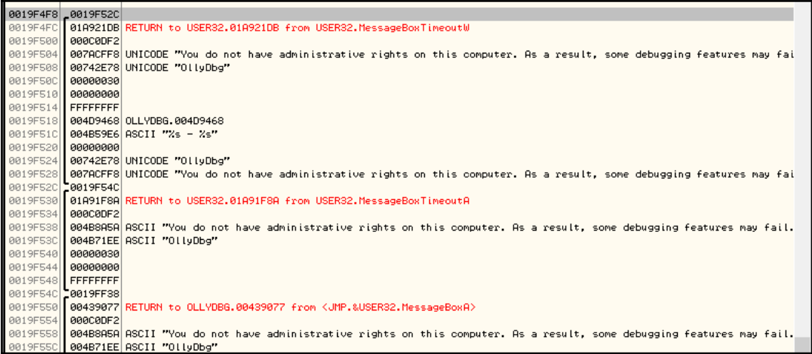
Figure 10: Stored values followed by a return address in OllyDbg
