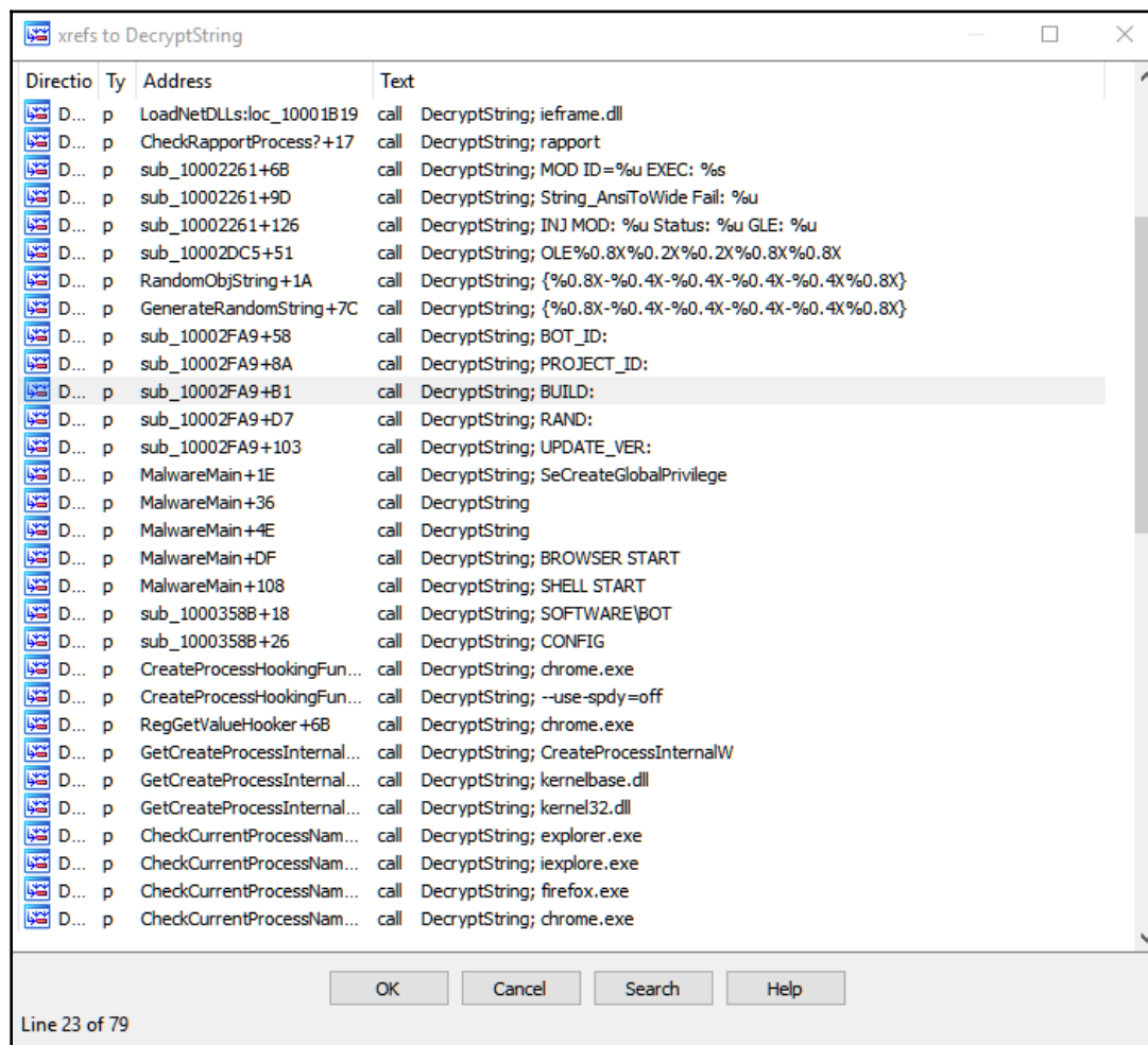
Figure 32: Xrefs to decryption routine in Vawtrak malware
