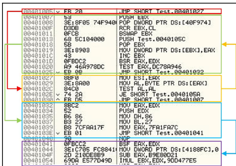
Figure 10: Code transportation with unconditional jumps
