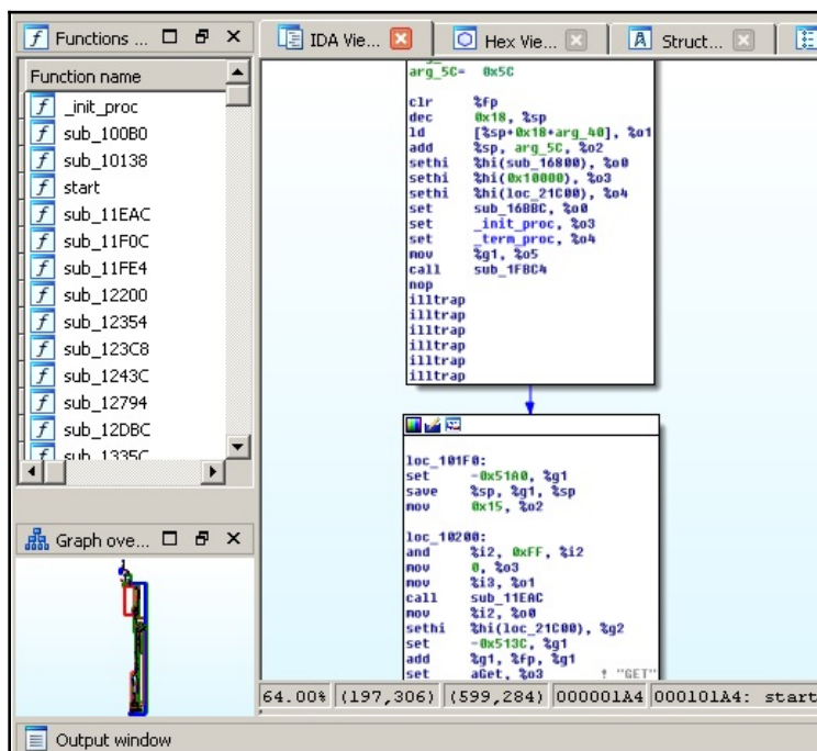
Figure 10: IDA processing a Mirai clone for SPARC architecture
