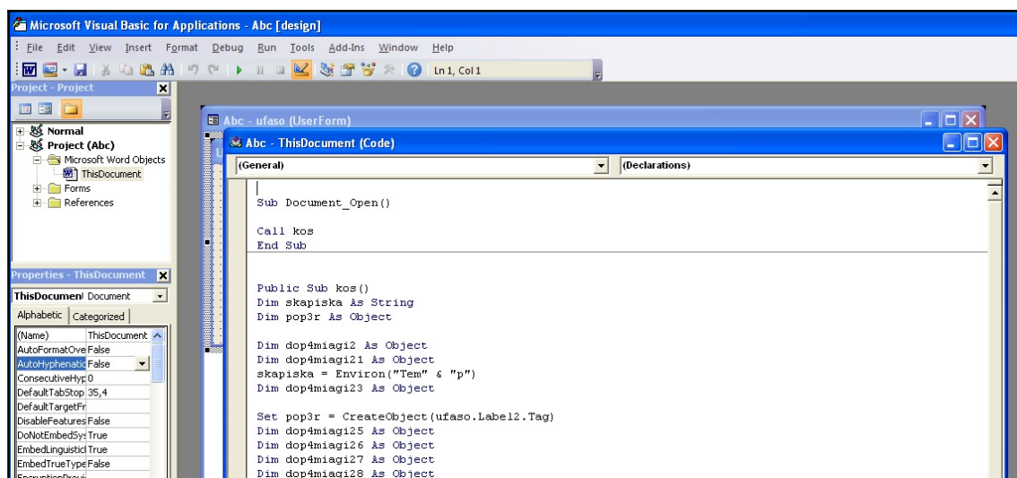
Figure 7: An example of a malicious macro inside a document
