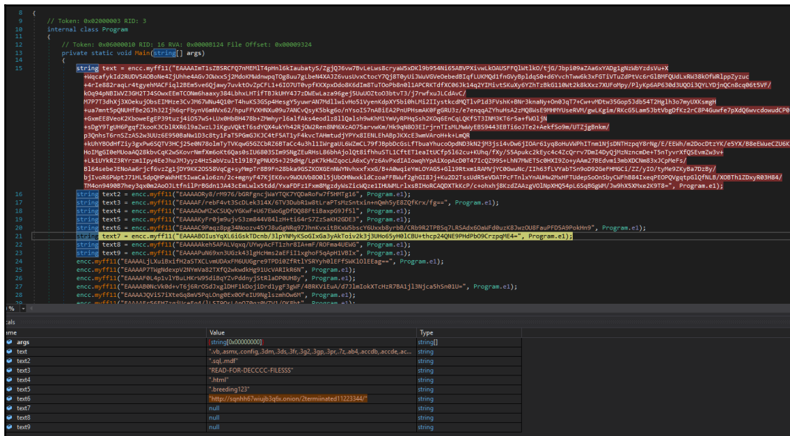
Figure 10: Samsam ransomware encrypted strings getting decrypted in memory
