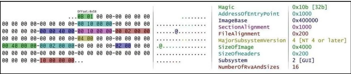
Figure 3: Optional header explained
