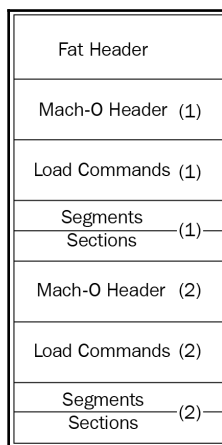
Figure 2: A fat Mach-O executable file
