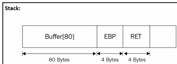
Figure 1: Local variable representations in the stack
