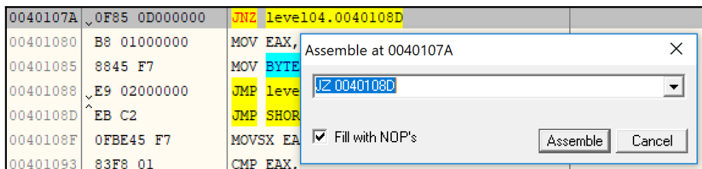
Figure 26: Working with assembly in OllyDbg
