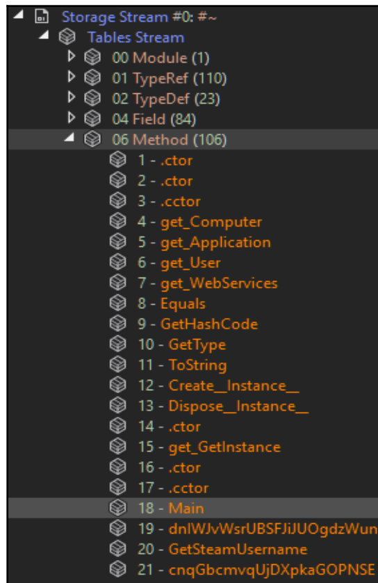
Figure 3: The EntryPoint method in the methods table in the first stream, #-
