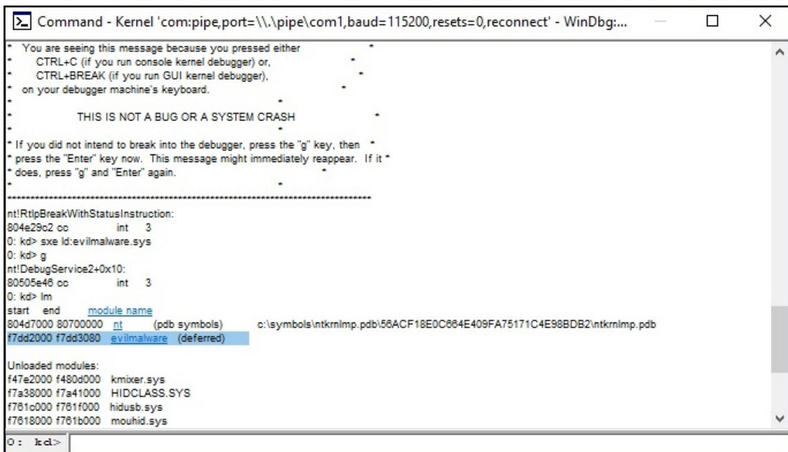
Figure 23: Breaking when a particular module is loading
