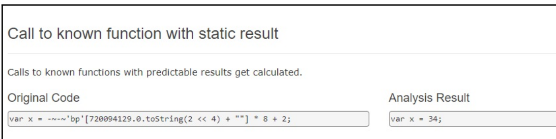
Figure 17: The JSDetox website describing functionality
