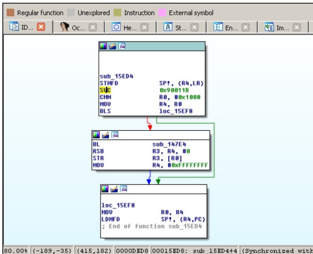
Figure 2: Mirai clone compiled for the ARM platform using the connect syscall
