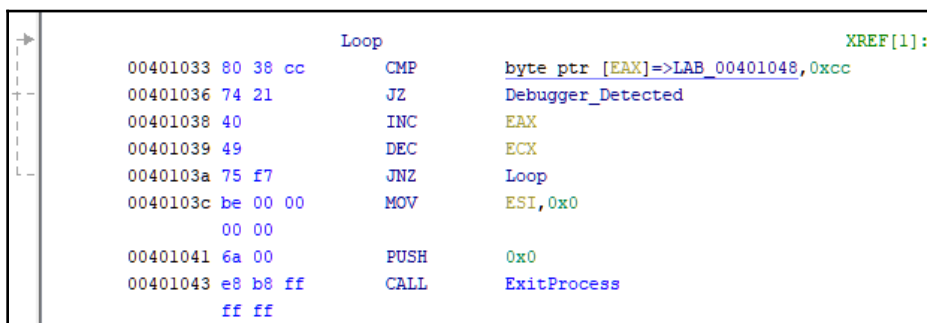
Figure 2: Simple INT3 scan
