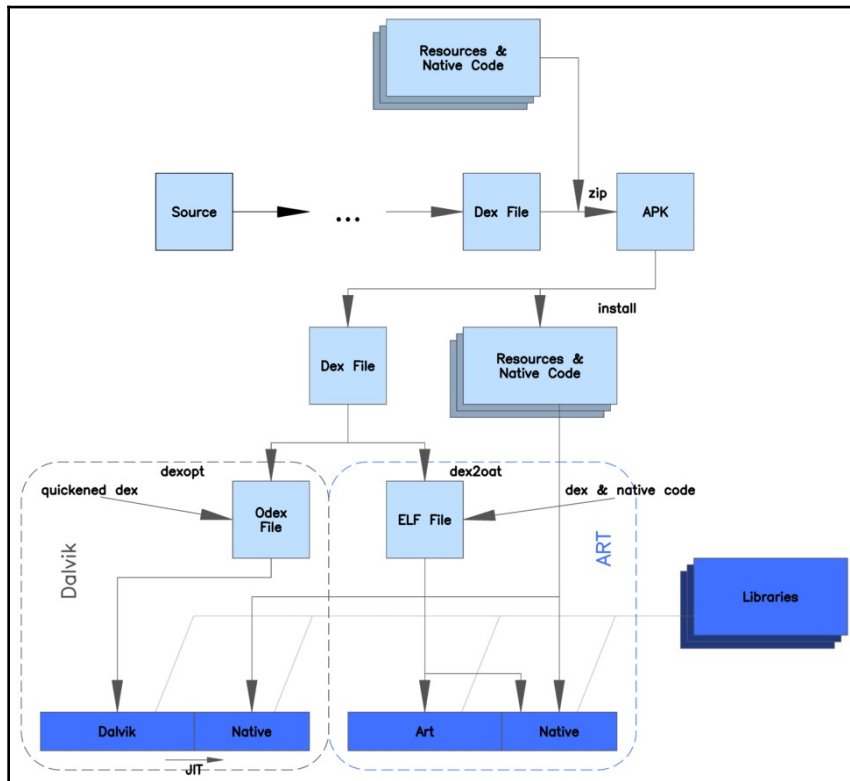
Figure 4: Diagram describing the differences between Dalvik and ART
