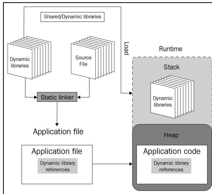
Figure 8: Dynamic linking from compilation to loading
