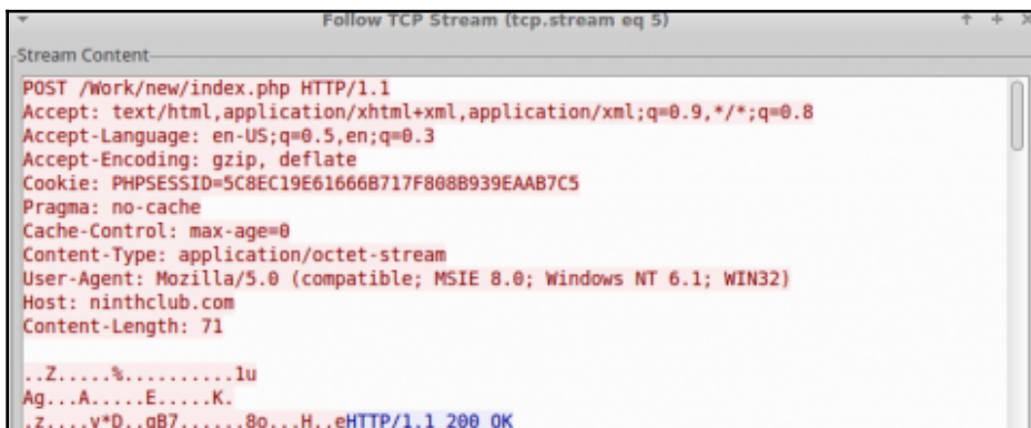
Figure 33: Network traffic of the Vawtrak malware
