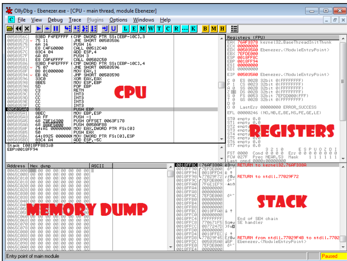
Figure 19: OllyDbg default window layout explained
