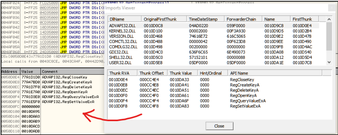
Figure 18: Import table before and after PE loading
