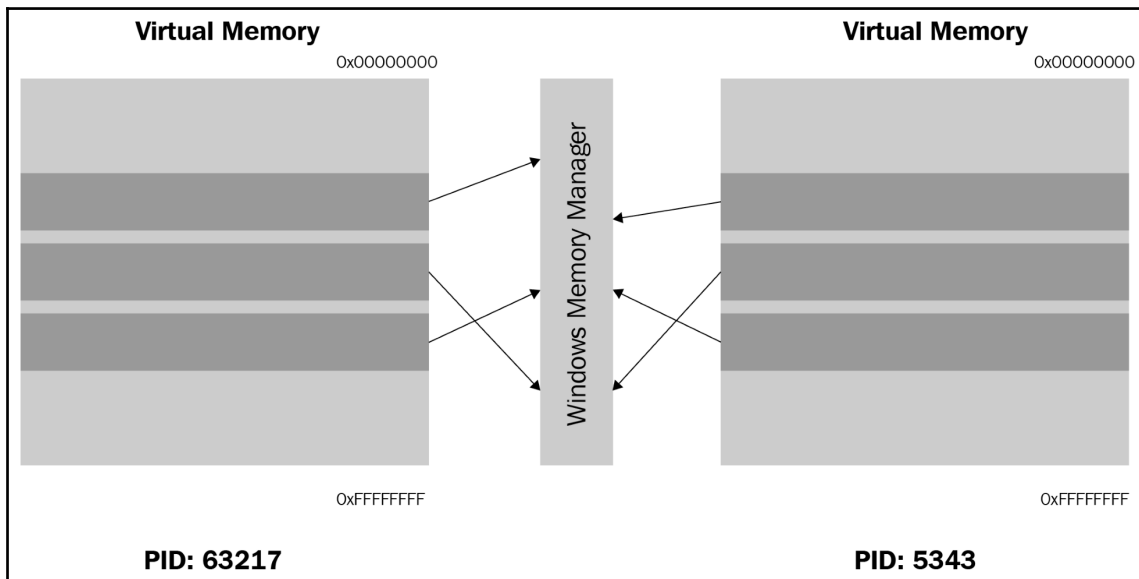
Figure 11: Mappings between physical and virtual memory
