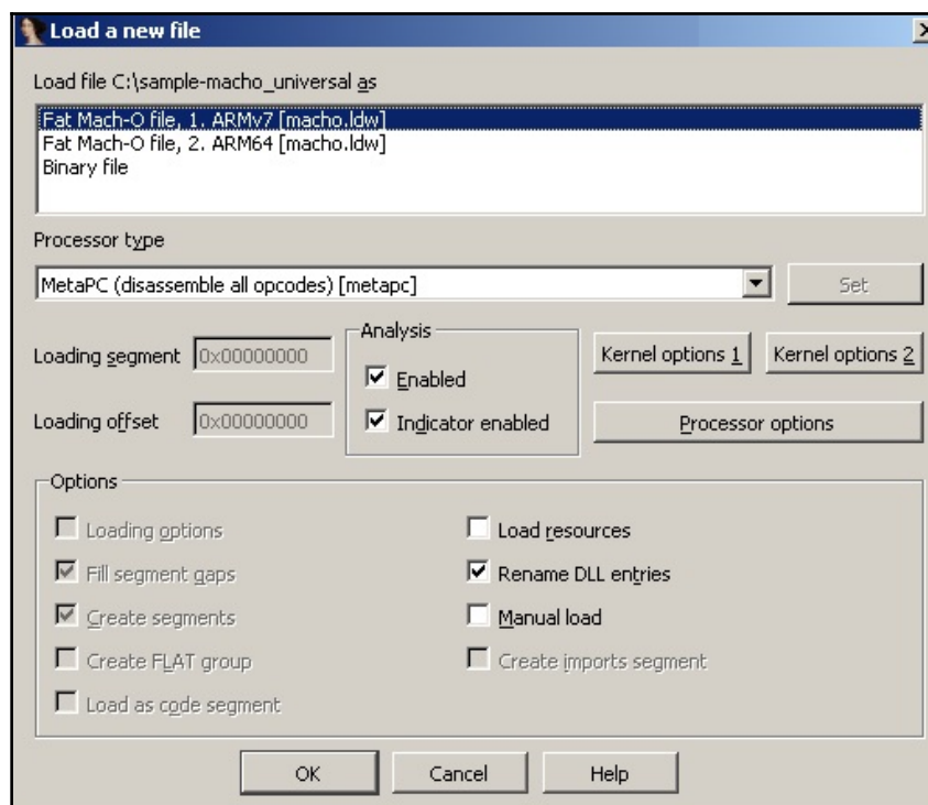
Figure 3: IDA confirming which thin Mach-O file in the fat binary should be analyzed
