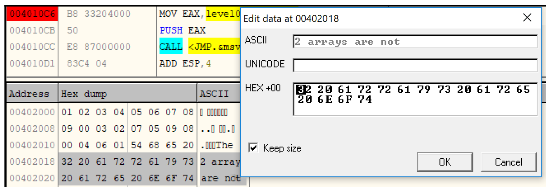
Figure 27: Data editing in OllyDbg
