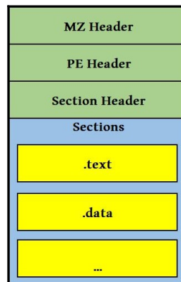
Figure 1: Example PE structure
