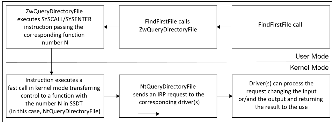
Figure 4: The API call life cycle
