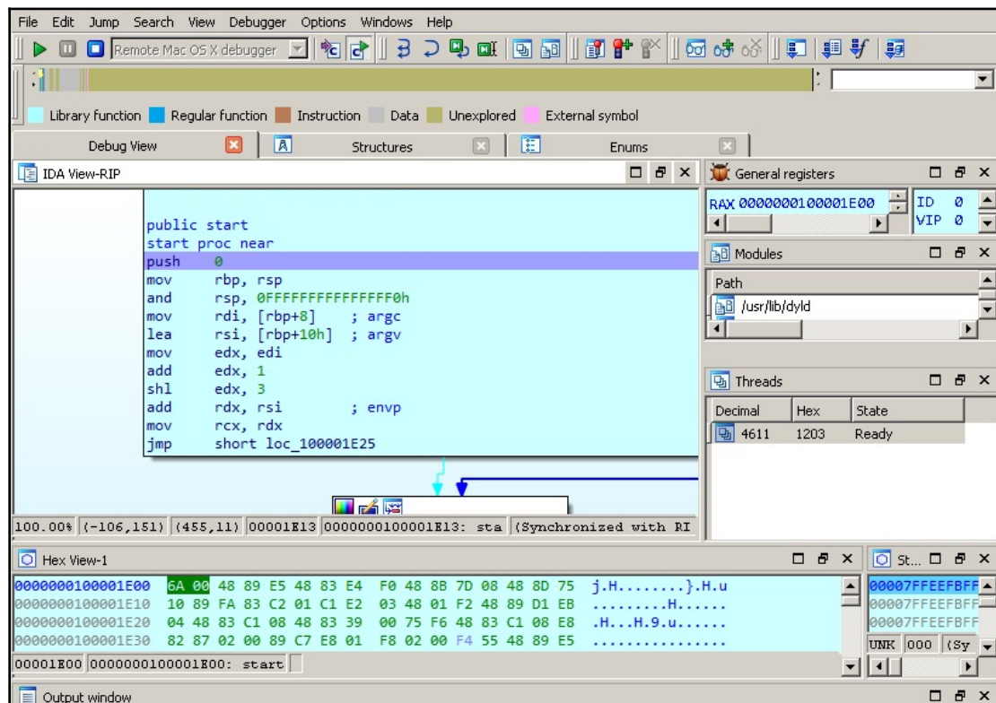
Figure 7: Debugging WireLurker malware targeting macOS remotely in IDA located on a Windows machine
