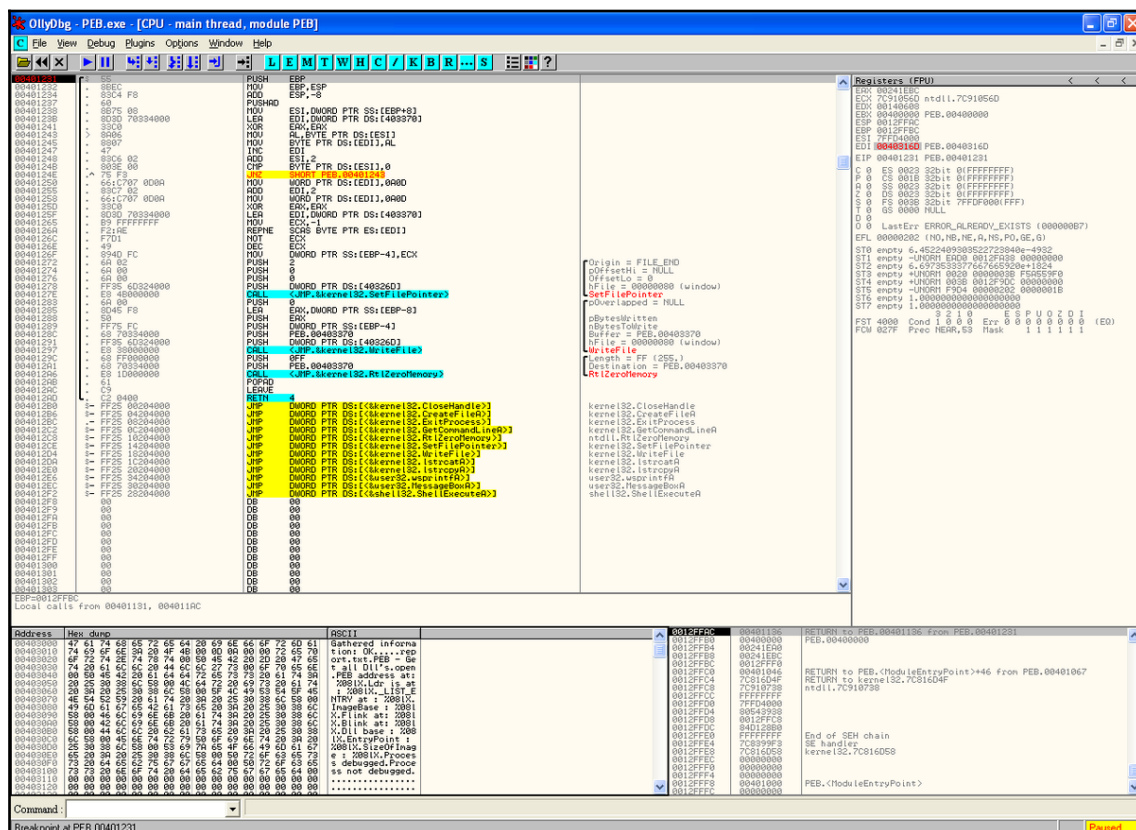
Figure 15: OllyDbg UI
