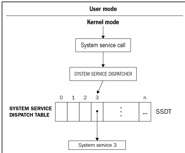
Figure 5: SSDT explained
