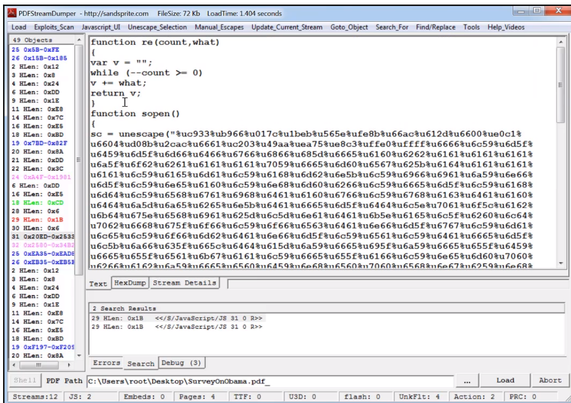
Figure 12: PDFStreamDumper tool
