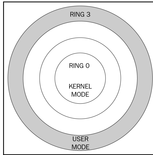
Figure 1: Processor rings
