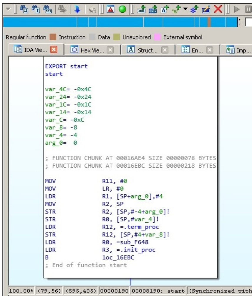
Figure 5: Disassembled IoT malware targeting ARM-based devices
