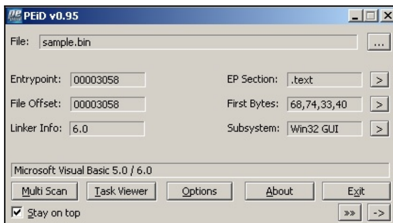
Figure 13: PEiD identifying Visual Basic
