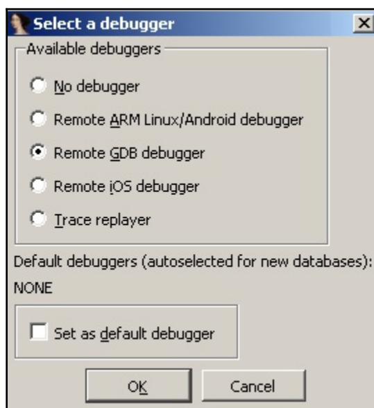
Figure 12: Available debuggers for the 32-bit ARM sample in IDA
