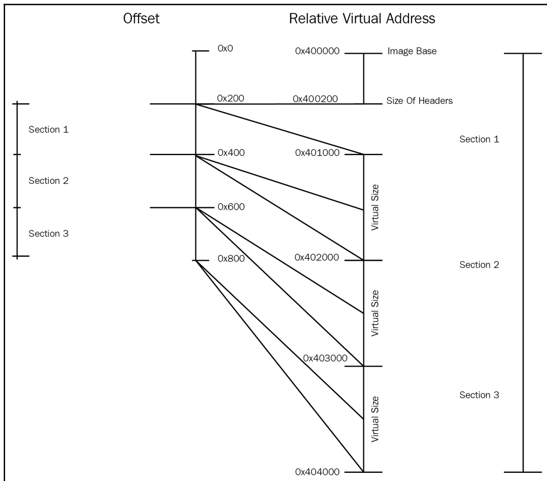
Figure 13: Mapping sections from disk to memory
