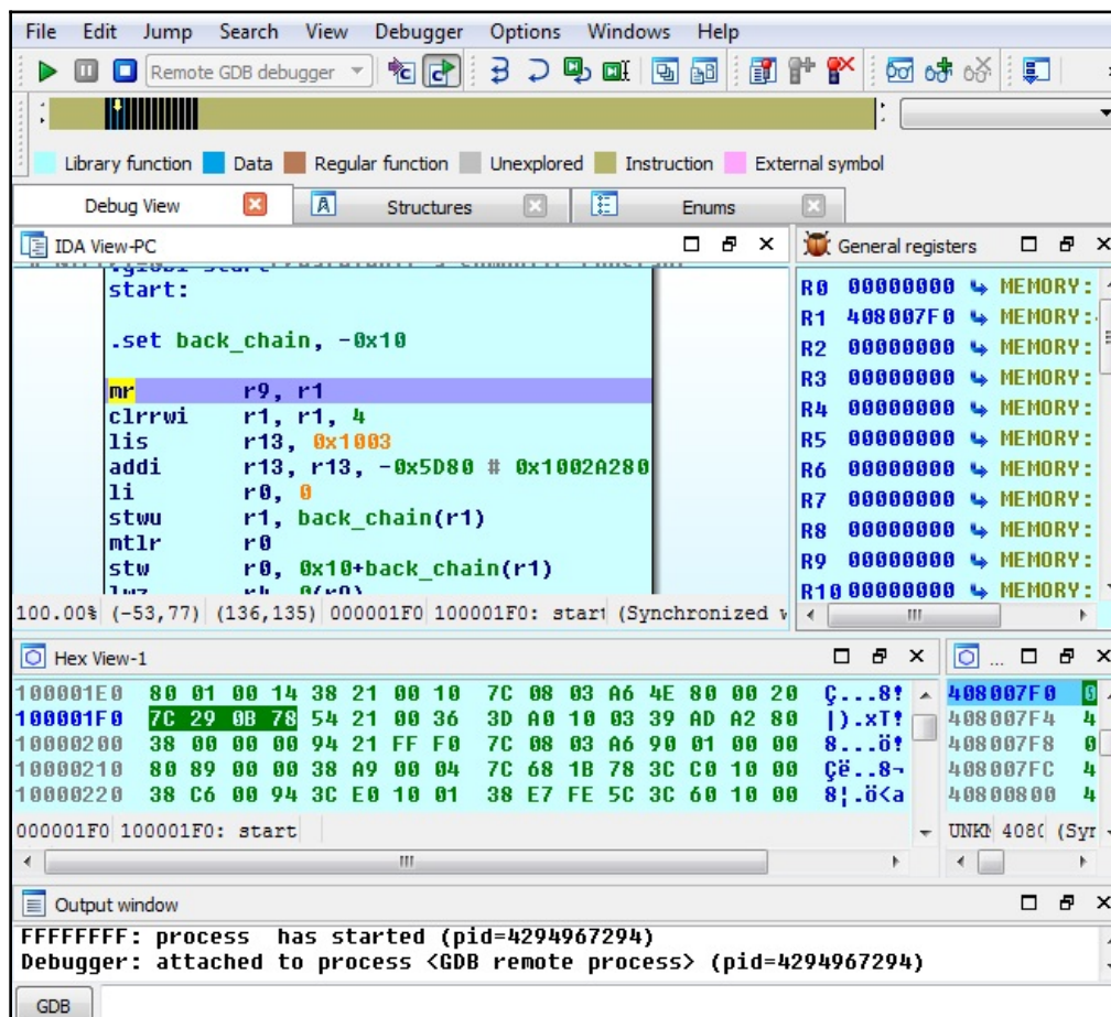
Figure 13: Debugging Mirai sample built for PowerPC in IDA on Windows via a remote qemu GDB server running on the x86 VM
