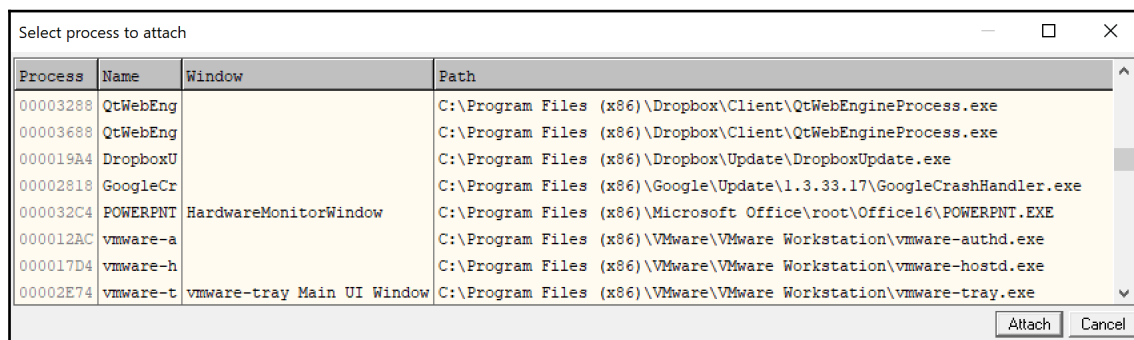
Figure 18: OllyDbg attaching dialog window
