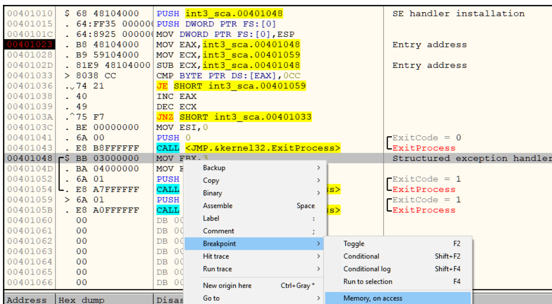
Figure 3: Breakpoint on Memory, On Access on the code section to detect INT3 scan loop/checksum calculating loop
