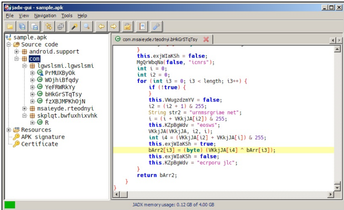
Figure 10. Decompiled Android sample in JADX
