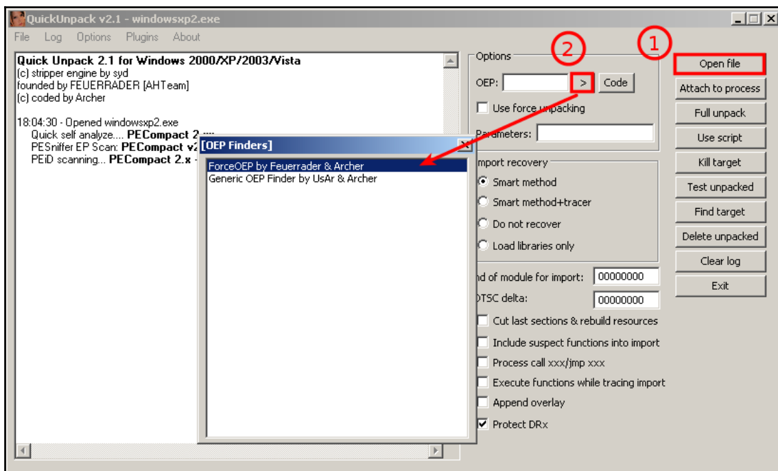
Figure 5: The QuickUnpack tool in detail
