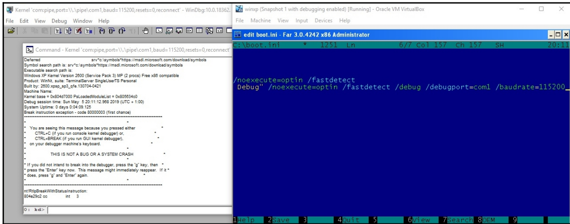
Figure 21: Kernel-mode debugging with VirtualBox and WinDbg over port COM
