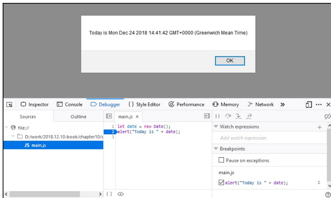
Figure 15: An example of the external JS script in Firefox Developer tools
