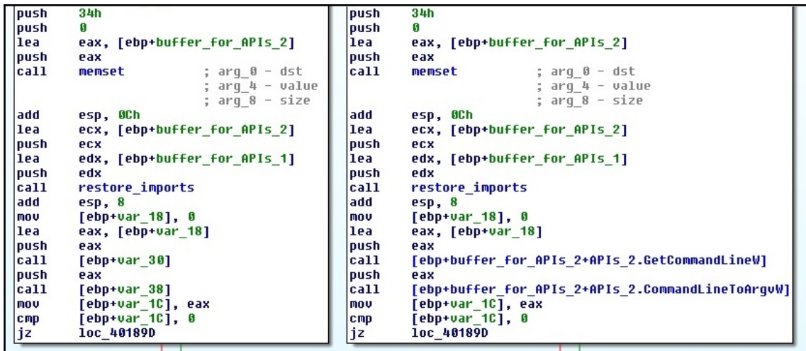
Figure 36: Mapping a local variable to the corresponding structure field
