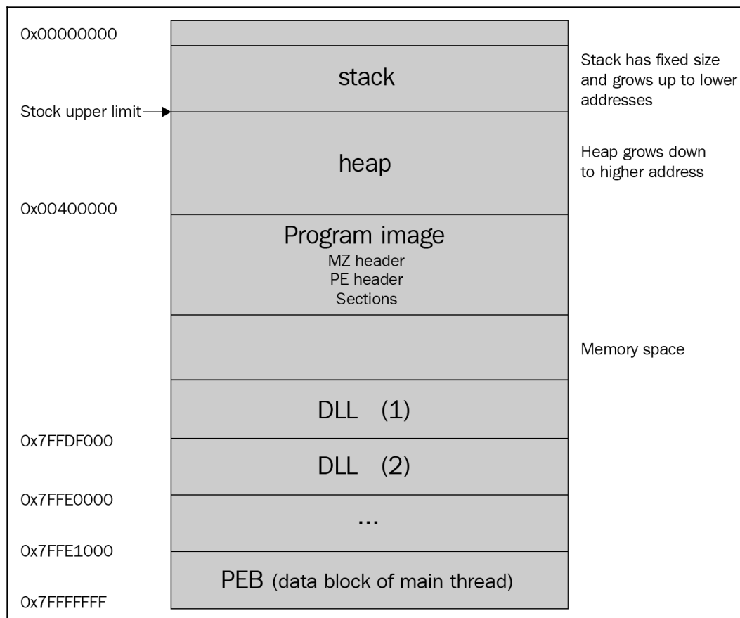
Figure 10: Example of a 32-bit process memory layout
