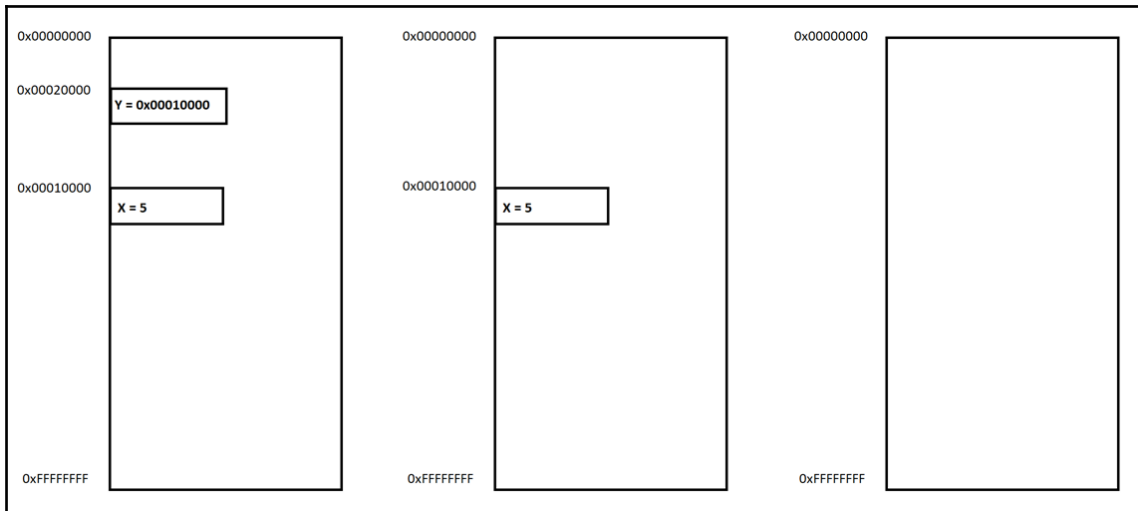
Figure 1: Virtual memory addresses
