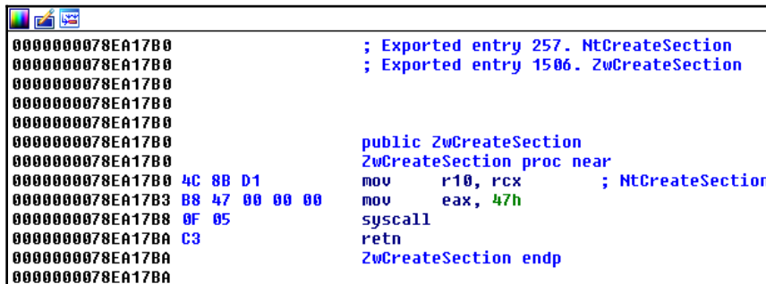
Figure 3: The syscall instruction
