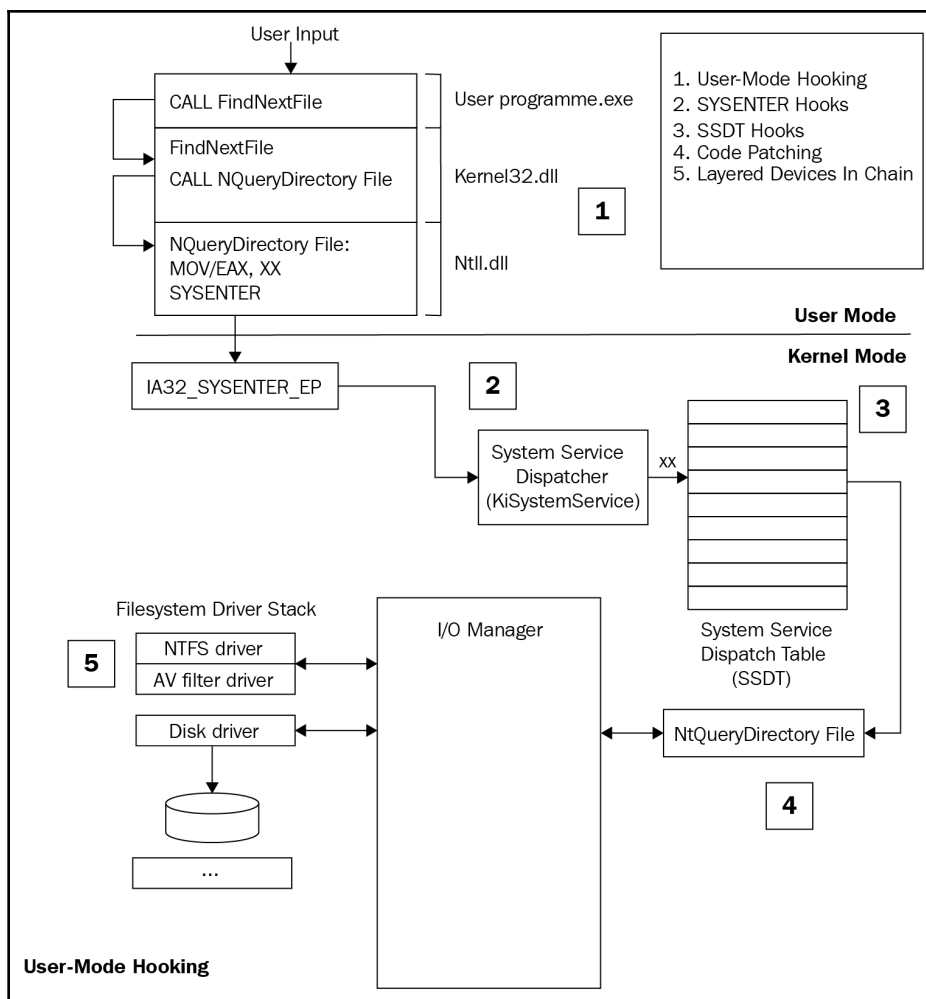
Figure 6: The hooking mechanisms of rootkits
