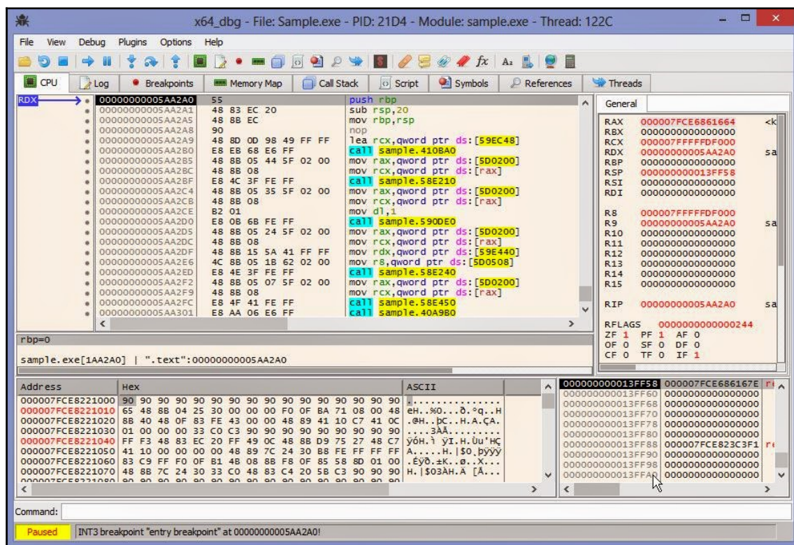
Figure 17: x64dbg UI
