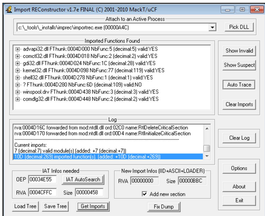
Figure 20: ImpREC interface
