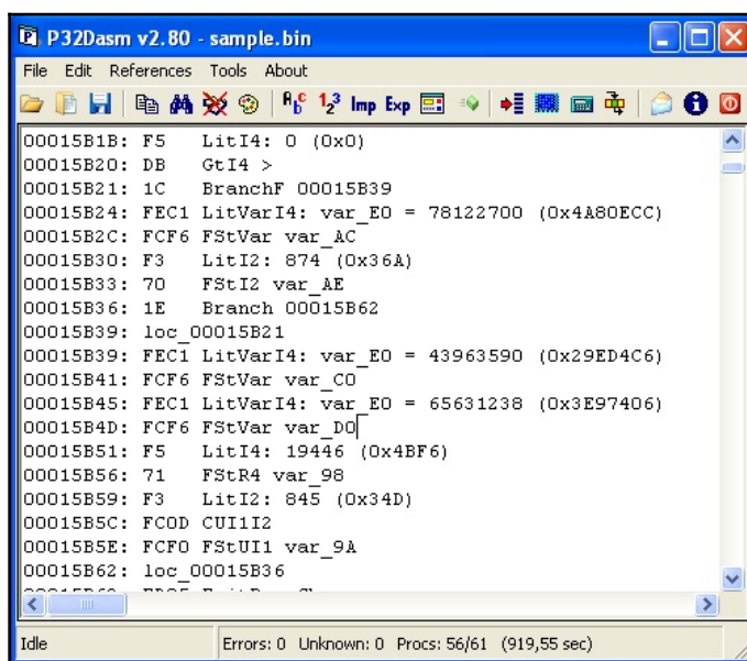
Figure 19: P32Dasm in action
