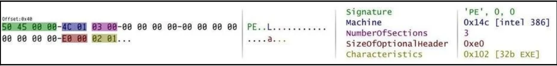
Figure 2: File header explained
