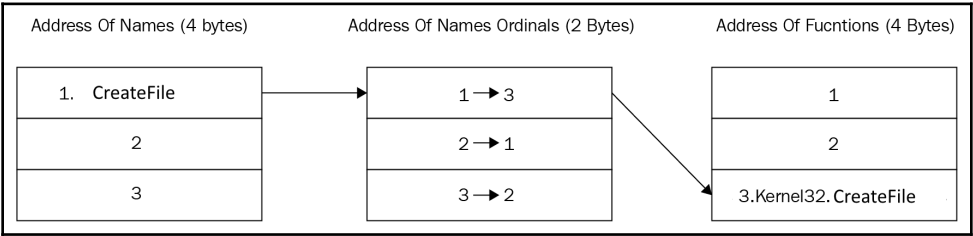
Figure 6: Export table structure (the numbers here are not real and have been provided as an example)
