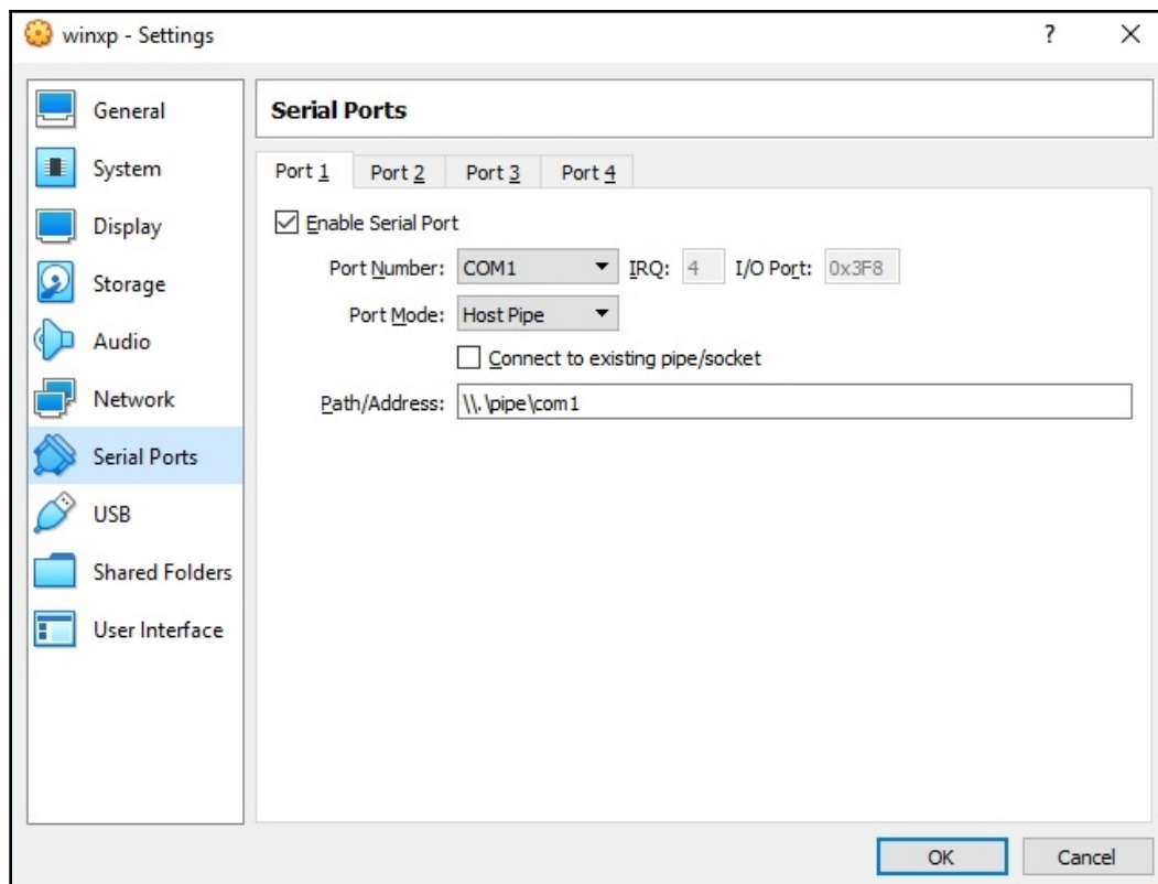
Figure 20: The VirtualBox setup for kernel-mode debugging over the COM port
