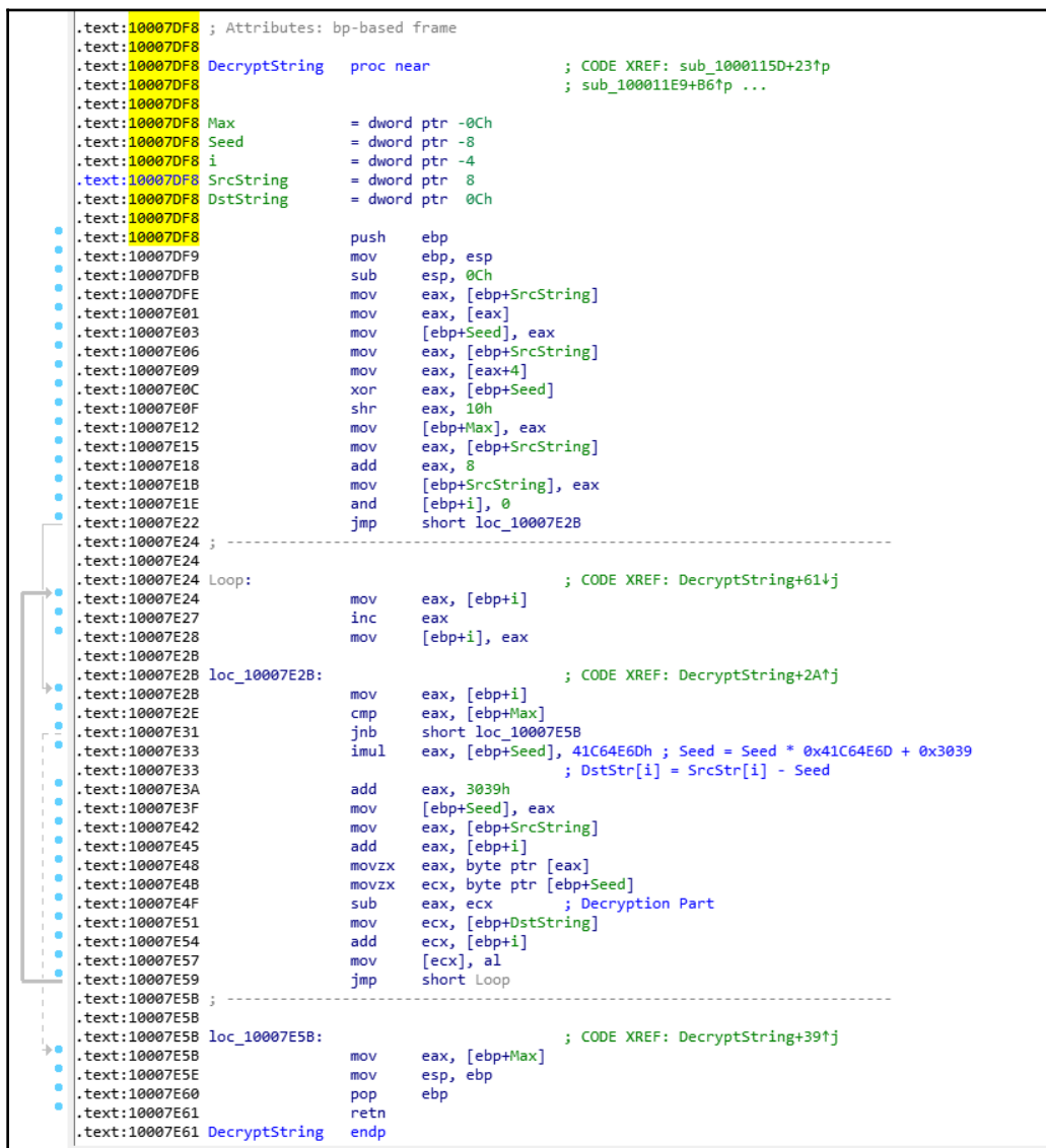
Figure 30: Encryption loop in Vawtrak malware
