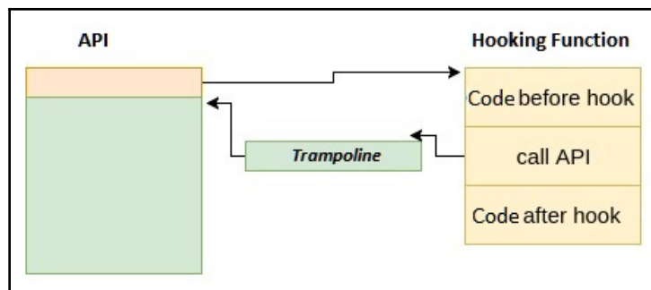
Figure 17: Hooking function with Trampoline
