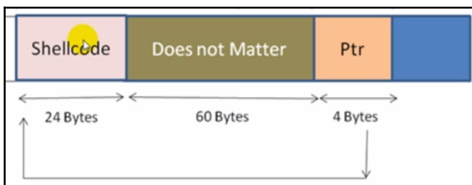
Figure 2: Overwriting Buffer[80] and the return address with shellcode
