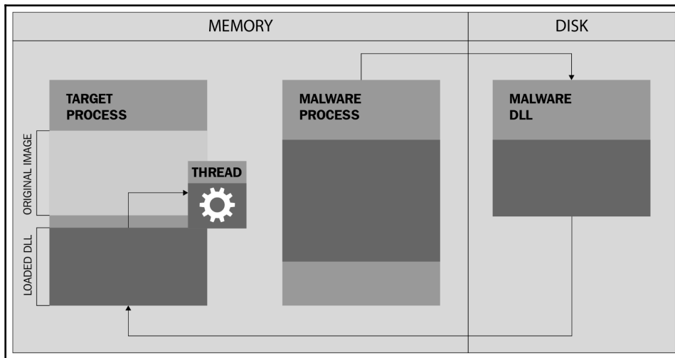
Figure 3. Simple DLL injection mechanism
