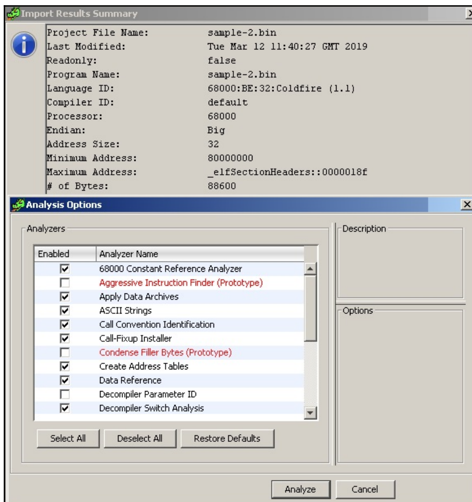
Figure 6: Multiple analysis options in Ghidra
