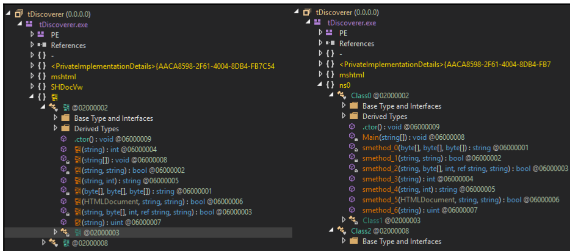
Figure 9: Hammerduke sample before and after running de4dot to deobfuscate the names
