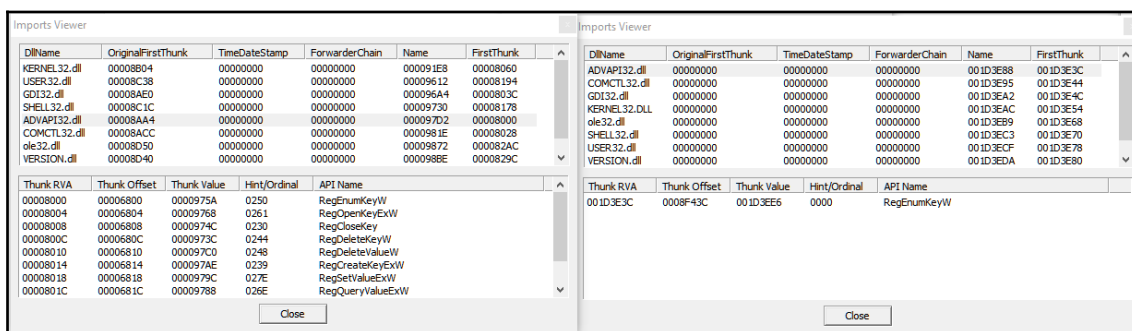
Figure 4: The import table of an unpacked sample versus a packed sample with UPX
