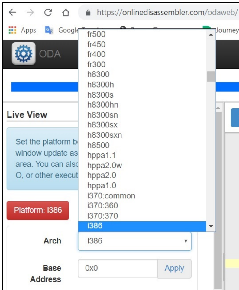
Figure 4: List of architectures supported by ODA
