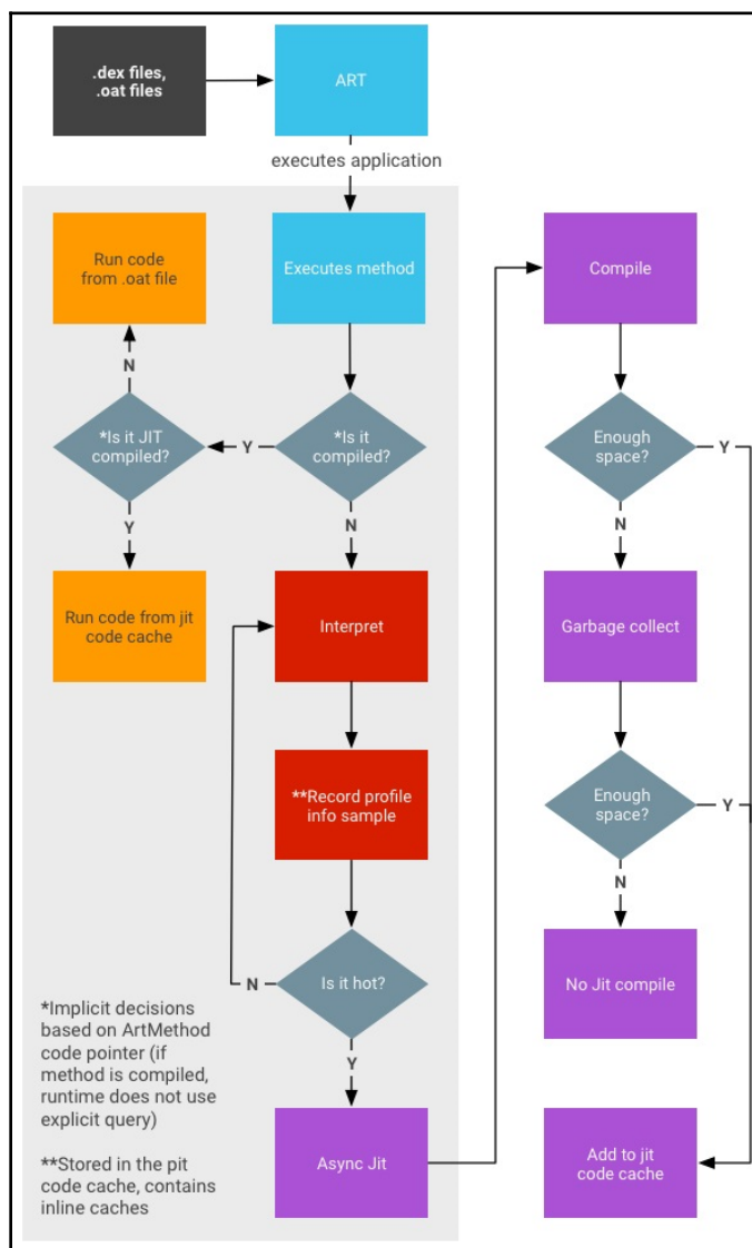
Figure 5: The process of compiling and executing files in ART
