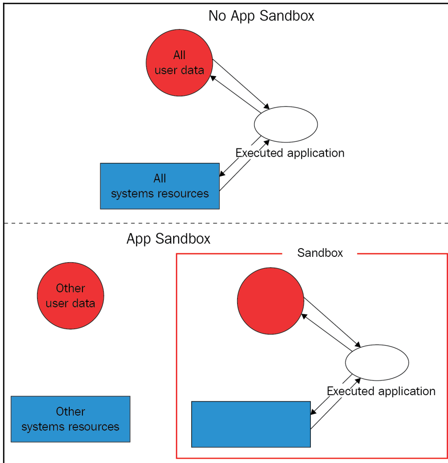
Figure 1: App Sandbox explained
