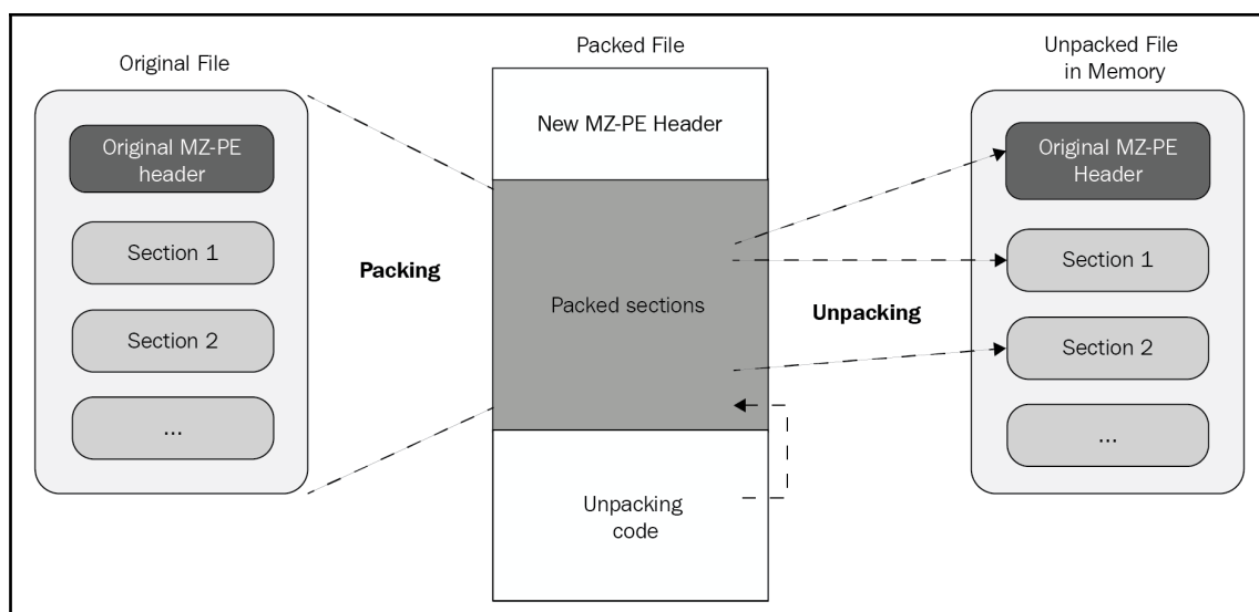
Figure 1: The process of unpacking a sample
