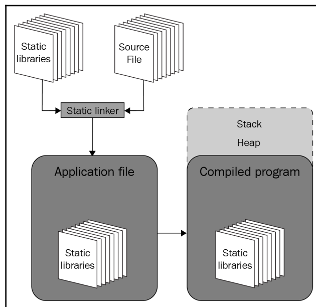
Figure 7: Static linking from compilation to loading
