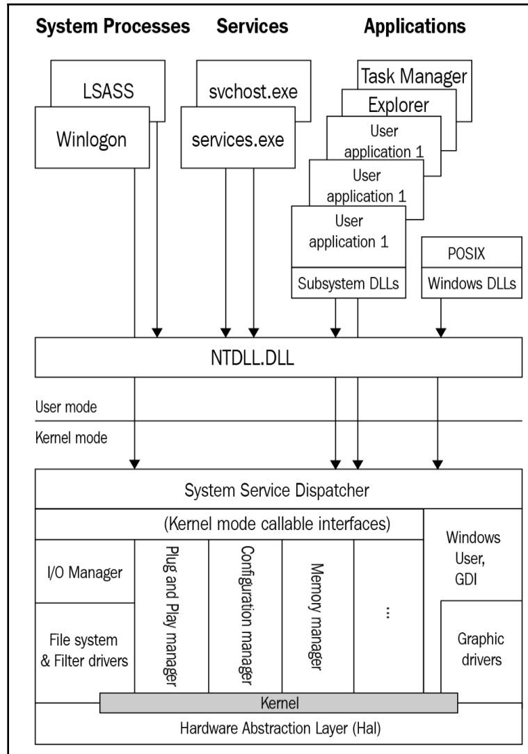
Figure 2: The Windows OS design
