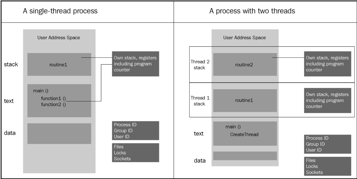
Figure 12: Example processes with one and multiple threads
