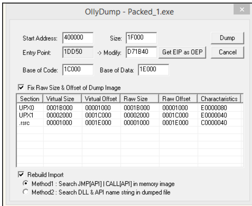
Figure 16: OllyDump UI
