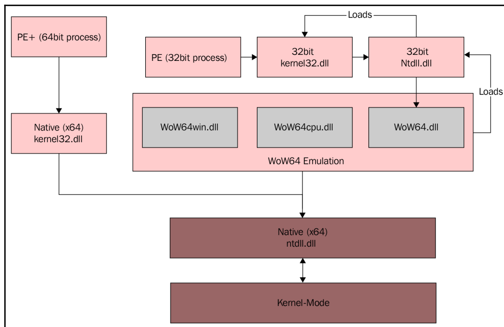
Figure 14: WOW64 architecture
