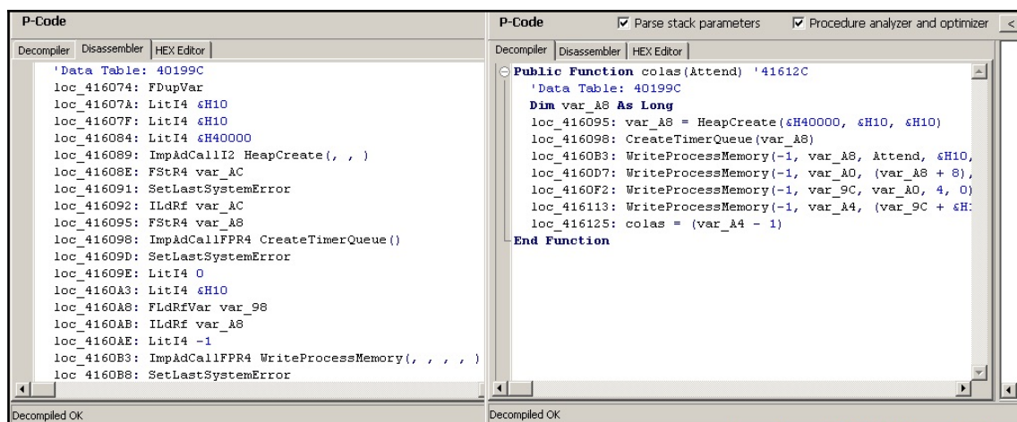
Figure 18: The same p-code function in VB Decompiler disassembled and decompiled
