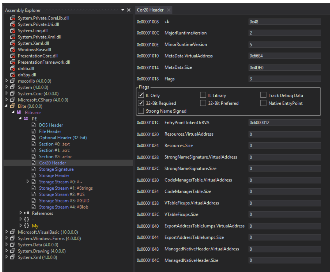
Figure 2: CLR header (COR20 header) and CLR streams
