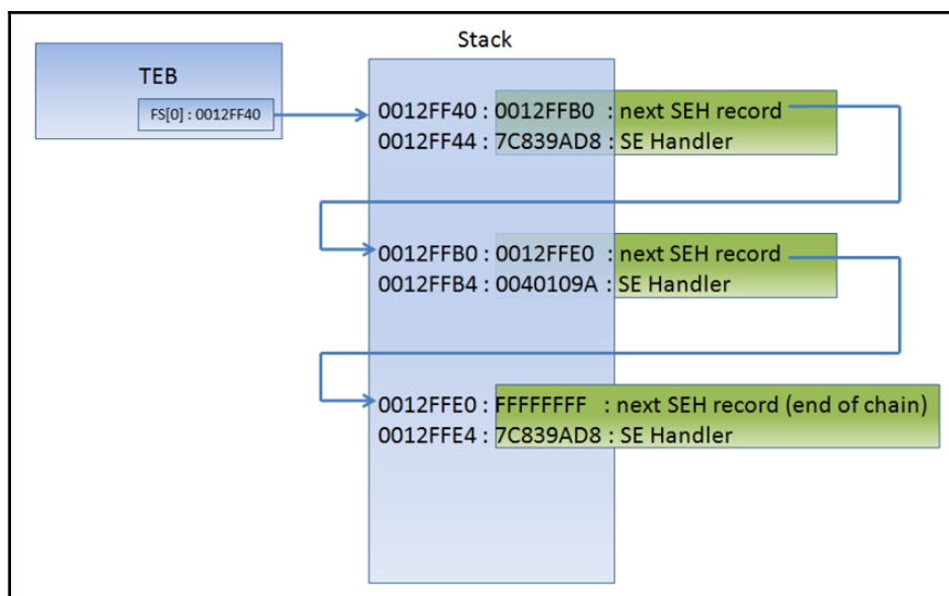
Figure 6: SEH linked list in the stack
