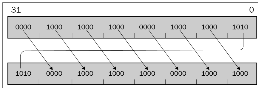
Figure 23: Example of the rol operation
