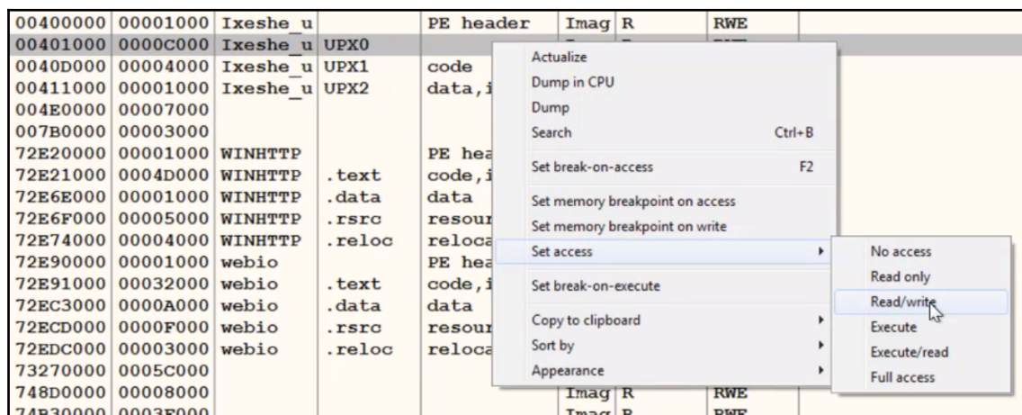
Figure 6: Changing memory permissions in OllyDbg
